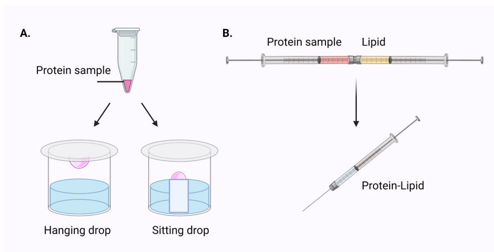
Figure 6. Schematic representation of vapor diffusion crystallization and LCP crystallization. A. Detergent solubilized protein sample is mixed with crystallization buffer and crystallization drops are set either as hanging drop or sitting drop. B. Detergent solubilized protein sample is mixed with lipid using two Hamilton syringes and a coupler and afterward protein-lipid mixture drop is set overlayed with buffer on a glass sandwich LCP plates. The figure was generated using BioRender.
