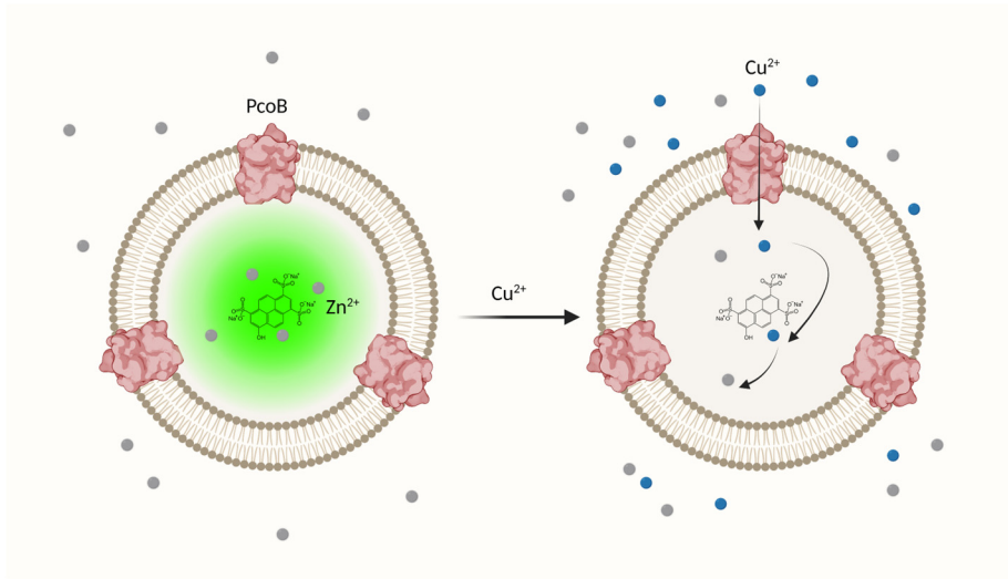
Figure 7. Schematic view of PcoB reconstitution into liposomes. Liposomes are formed with fluorophore dye trapped inside. PcoB is reconstituted into liposomes and through addition of \text{Cu}^{2+} containing buffer, quenching of the dye is measured as a result of \text{Cu}^{2+} import via the PcoB channel. The figure was generated using BioRender.
