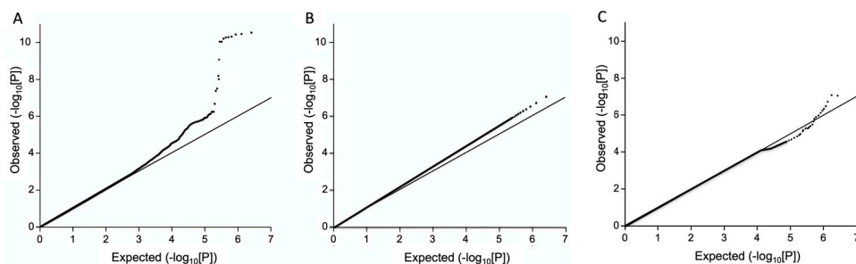
Figure 6. Quantile-quantile (QQ) plot of simulated data from a genome-wide association study (GWAS). A) QQ plot where the observed values generally correspond to the expected values, with the exception from variants associated with the investigated trait. B) QQ plot showing an early separation of the observed from the expected, suggesting e.g., population stratification. C) QQ plot with a section of deflated values which could indicate a too low MAF threshold in the GWAS. A and B adapted from Ehret et al. (2010) with permission from Springer Nature (license number: 5478670327871).
