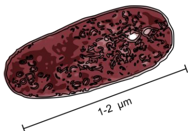
Figure 2. Purple and green photosynthetic bacteria
