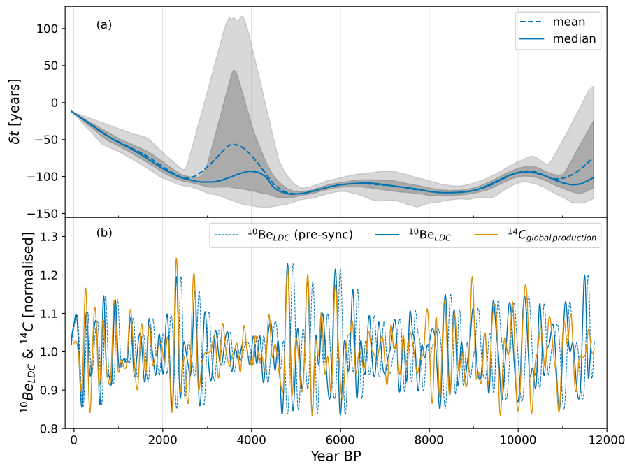
Figure 3.4: (a) Timescale transfer function with envelopes of 50% CI (dark grey) and 95% CI (light grey). \delta t indicates the age difference between t_{\text{IntCal20}} and t_{\text{LDC}} , i.e. t_{\text{IntCal20}} - t_{\text{LDC}} . (b) A comparison of the variations at timescales between 150 – 500 years of LDC ^{10}\text{Be} and ^{14}\text{C} production rate before and after the synchronisation. Noted that the LDC timescale before the synchronisation is based on the EDC age-to-depth relationship (Veres et al., 2013) stretched by 8% (see text).
