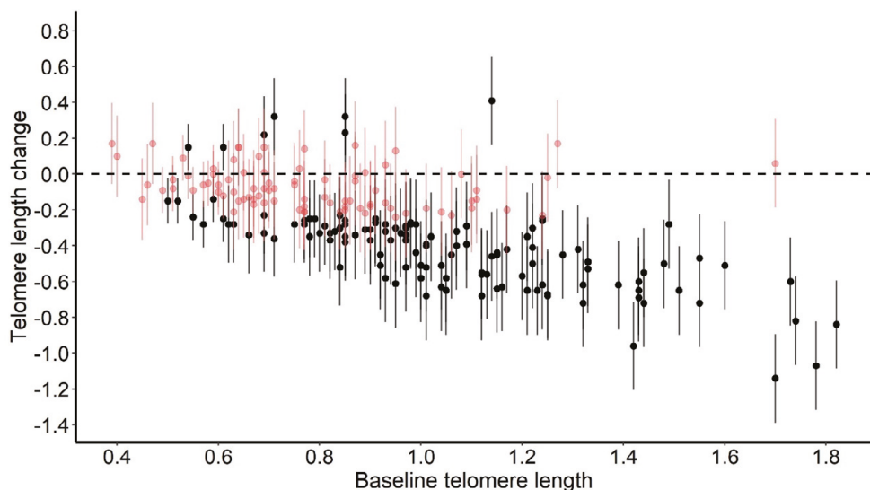
Figure 11. Example dataset of change in telomere length (TL; measured as T/S ratio) of great reed warblers. Negative values represent the shortening of TL and positive values indicate TL elongation. Error bars represent estimated measurement errors of TL change for the sample ( \pm 2 \times \text{SD} ). Samples in light shading in red are those where the 2 \times \text{SD} error bar overlaps TL change = 0 (for more details see Chapter IV).
