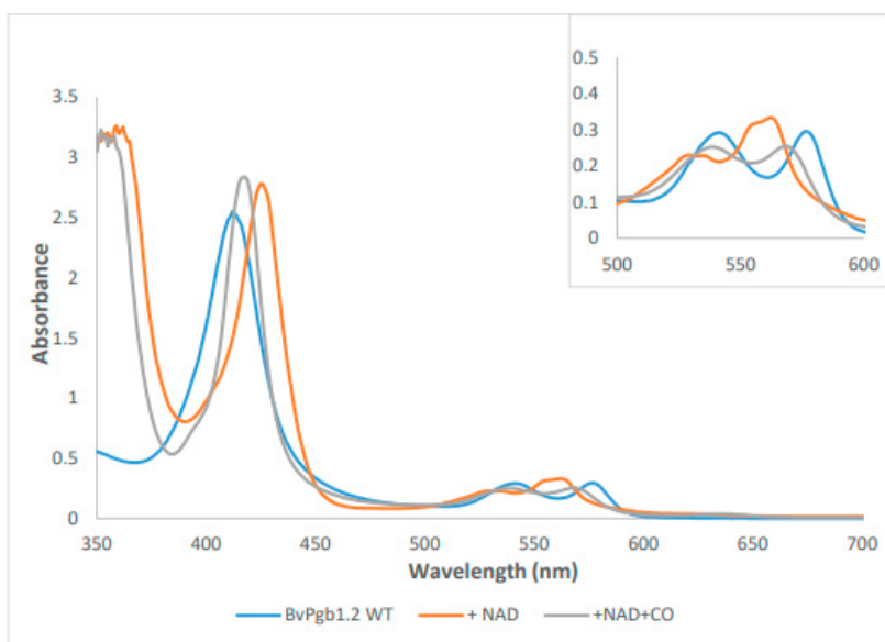
Figure 6. UV-Vis spectrum for oxygenated (blue), reduced (orange) and CO-saturated (gray) recombinant BvPgb1.2. The protein was expressed and purified as described above. The shift in Soret and heme peaks for the different states/ligands indicate a functional globin.
