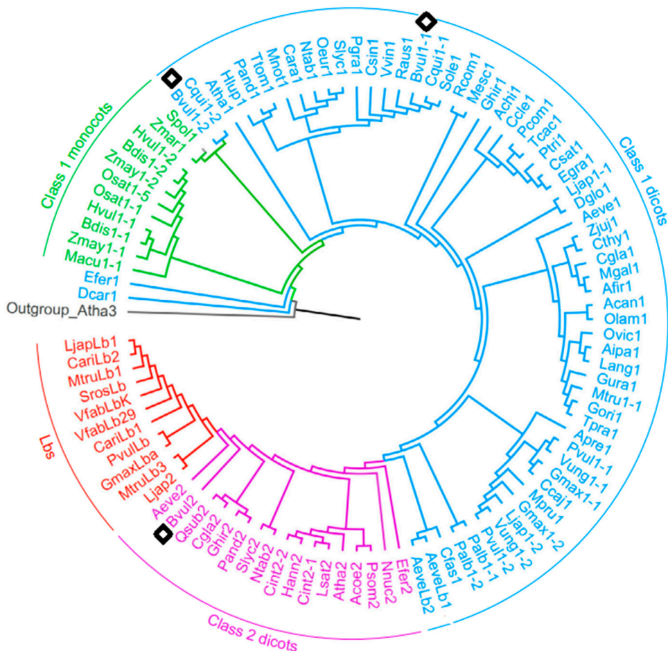
Figure 7. Phylogenetic tree of globin origin for class I nsPgbs in monocots (green), class I and II in dicots (blue and purple, respectively) and sPgbs (Lbs) in legumes (red). The transitions from class I to class II nsPgbs and later to sPgbs (Lbs) were observed. The absence of class II nsPgbs in monocots is also evident. Atha3 was used as outgroup and the majority of bootstrap values were close to 100% except Efer1/Dcar1 branches (<70%). Adopted and modified from [44].
