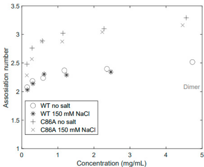
Figure 20. Association number of BvPgb1.2 WT and C86A as a function of protein concentration, where 1 = 19.2 kDa (molecular weight of monomer). The molecular weight of the dimer is equivalent to association number 2. Size distributions for WT and C86A were between 39-48 kDa and 48-63 kDa, respectively. The last point for WT+150 mM NaCl (4.6 mg/ml) was not included due to radiation damage.
