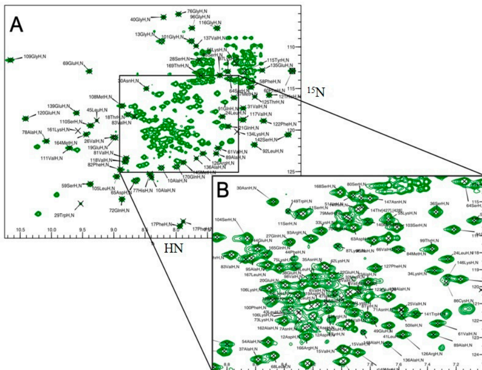
Figure 15. (A): 1 H- 15 N TROSY spectrum for cyanide-bound BvPgb1.2. (B): Zoom-in depiction of residue-rich section of the spectrum. These spectra are a complement to the information in Table 3. The spectrum regarding the paramagnetic character of O 2 -bound BvPgb1.2 was not included here. Adopted and modified from [138] ( Paper II ).
