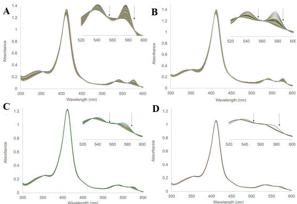
Figure 9. (A) and (B): Complete autoxidation spectra for BvPgb1.2 WT. (C) and (D): Complete autoxidation spectra for C86A mutant. The spectra were collected at 25 (A and C) and 37 °C (B and D), respectively. Adopted and modified from [95] (Paper I).
