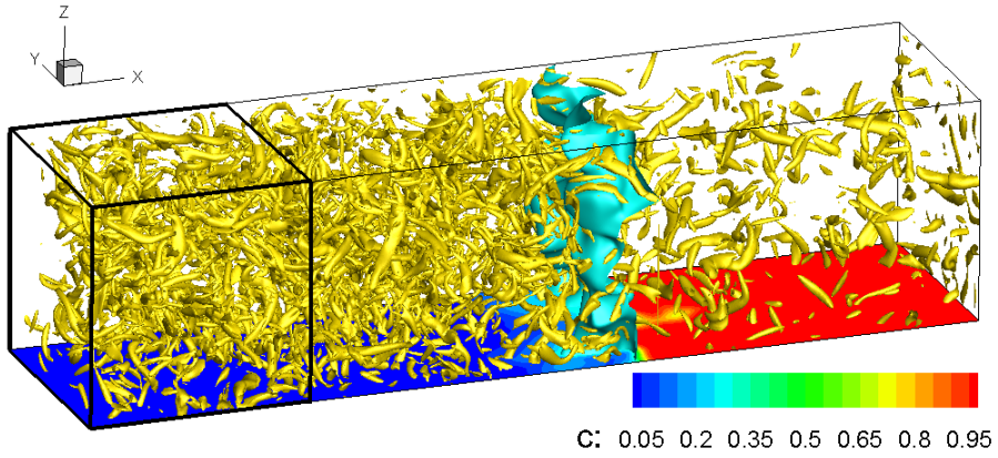
Figure 2.1: 3D snapshots of case B. The c -field is shown on the bottom plane with an isosurface of \hat{c} = 0.3 (cyan) and rotating flow structures are visualized using yellow iso-contours of the second eigenvalue of the flow strain rate tensor (also referred to as "Lambda2-vortex method" [128]).
