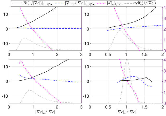
Figure 5.5: Fully developed [\phi]_s|_{1/|\nabla c|, \hat{c}} for three quantities \phi \in [\partial_t^*(1/|\nabla c|), \nabla \cdot \mathbf{u}/|\nabla c|, \mathcal{K}] (left axis) and \text{pdf}_s(1/|\nabla c|)|_{\hat{c}} (right axis). Results refer to \Theta = 2 (case B, top) and 7 (case D, bottom) at \hat{c}=0.3 (left) and 0.87 (right). All dimensioned quantities are normalized based on speed unit S_L and space unit \delta_F .
