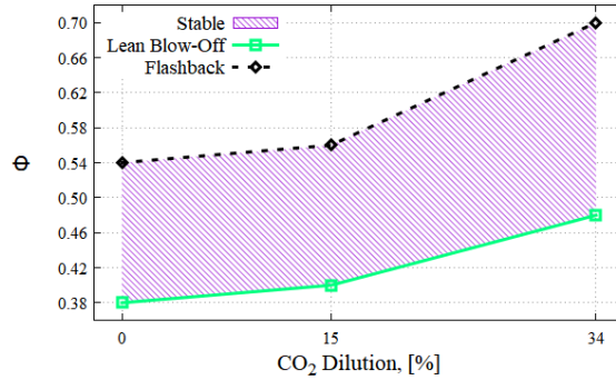
Figure 5.24: Operability limits for the three different \text{CO}_2 dilutions.
