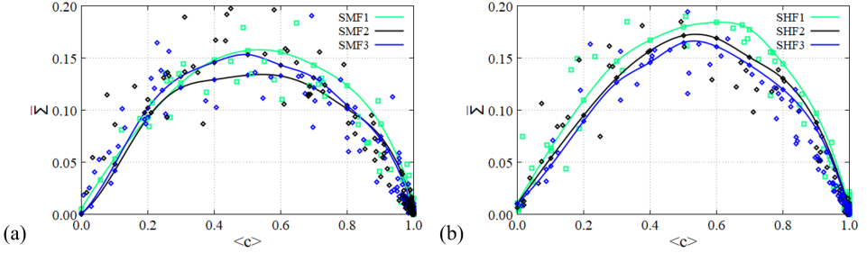
Figure 5.15: Mean flame surface density against mean progress variable for the stable \text{CH}_4/\text{air} flames (left) and \text{H}_2 -enriched \text{CH}_4/\text{air} flames (right).
