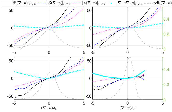
Figure 5.4: Fully developed [\phi]_s|_{\nabla \cdot \mathbf{n}, \hat{c}} for four quantities \phi \in [\partial_t^*(\nabla \cdot \mathbf{n}), \mathbb{B}(\nabla \cdot \mathbf{n}), \mathbb{A}(\nabla \cdot \mathbf{n}), \nabla \cdot \mathbf{u} \nabla \cdot \mathbf{n}] and \text{pdf}_s(\nabla \cdot \mathbf{n})|_{\hat{c}} (labeled on right axis). Results refer to \Theta = 2 (case B, top) and 7 (case D, bottom) at \hat{c}=0.3 (left) and 0.87 (right). All dimensioned quantities are normalized based on speed unit S_L and length \delta_F .
