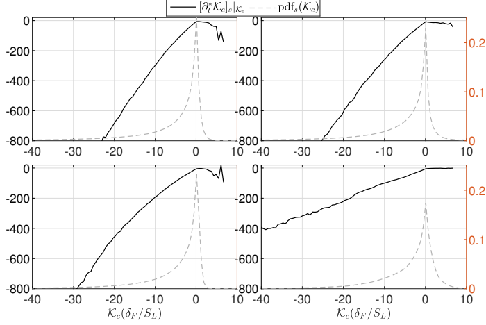
Figure 5.6: Fully developed [\partial_t^* \mathcal{K}_c]_s |_{\mathcal{K}_c, \hat{c}} (left axis) and \text{pdf}_s(\mathcal{K}_c) |_{\hat{c}} (right axis). RResults refer to \Theta = 2 (case B, top) and 7 (case D, bottom) at \hat{c}=0.3 (left) and 0.87 (right). All dimensioned quantities are normalized based on speed unit S_L and length \delta_F .
