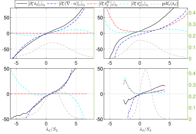
Figure 5.2: Fully developed [\partial_t^* \phi]_s |_{\tilde{s}_d, \hat{c}} for four quantities \phi \in (\tilde{s}_d, \nabla \cdot \mathbf{n}, \tilde{s}_d^W, \tilde{s}_d^n) (labeled on left axis) and \text{pdf}_s(\tilde{s}_d) |_{\hat{c}} (labeled on right axis). Results refer to \Theta = 2 (case B, top) and 7 (case D, bottom) at \hat{c} = 0.3 (left) and 0.87 (right). All dimensioned quantities are normalized based on speed unit S_L and length unit \delta_F .
