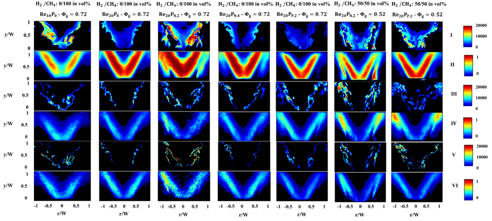
Figure 5.10: OH- and CH_2O -PLIF results for methane/air and hydrogen-enriched methane/air flames at stable flame conditions. From top row to bottom row: I single-shot of OH-PLIF; II PM of OH PLIF intensity; III single-shot of CH_2O -PLIF intensity; IV PM of CH_2O PLIF intensity; V heat release zone ( OH \times CH_2O ); VI PM of heat release zone.
