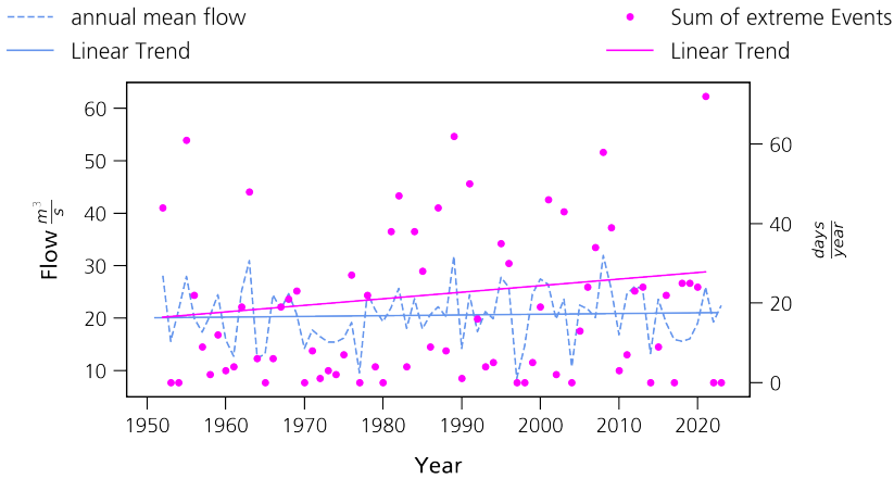
Figure 12: Annual average outflow and annual sum of extreme events (daily flow higher than 95 % of measurements) of Lake Bolmen measured at the hydropower plant in Skeeen
