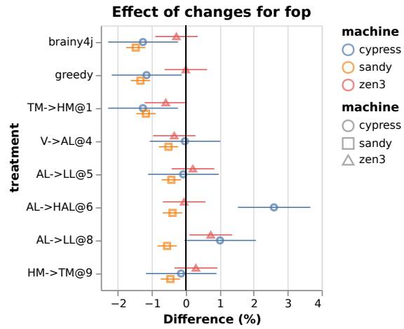
Figure 3: Effect of changes for bloat (a) and fop (b). Points denote the mean speedup, error bars denote the 95% confidence intervals. Greedy search finds an important optimization for bloat, but Brainy4J misses it. For fop, Greedy search and Brainy4J find a small optimization for Sandy and Zen3.
