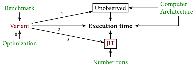
Figure 4: The SCM of influences on execution time in our experiments. “Computer Architecture” has the same meaning as in Figure 1. “Benchmark” now refers to the name of the benchmark. “Variant” refers to the result of applying the optimization to the benchmark and packaging it in a JAR. “Optimization” refers to the optimization applied to the program (e.g. “Original”, “CoCo”, “Greedy search”, etc.). We account for JIT-compilation by running the program several times, which is reflected in the “Number runs” variable.
