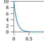
Figure 4: Exponential Distribution with mean at 0.1.
