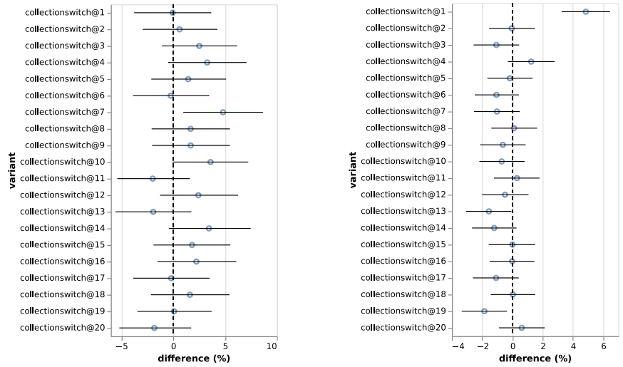
(a) For bloat , we could not find a positive effect from CollectionSwitch, on individual sites.
