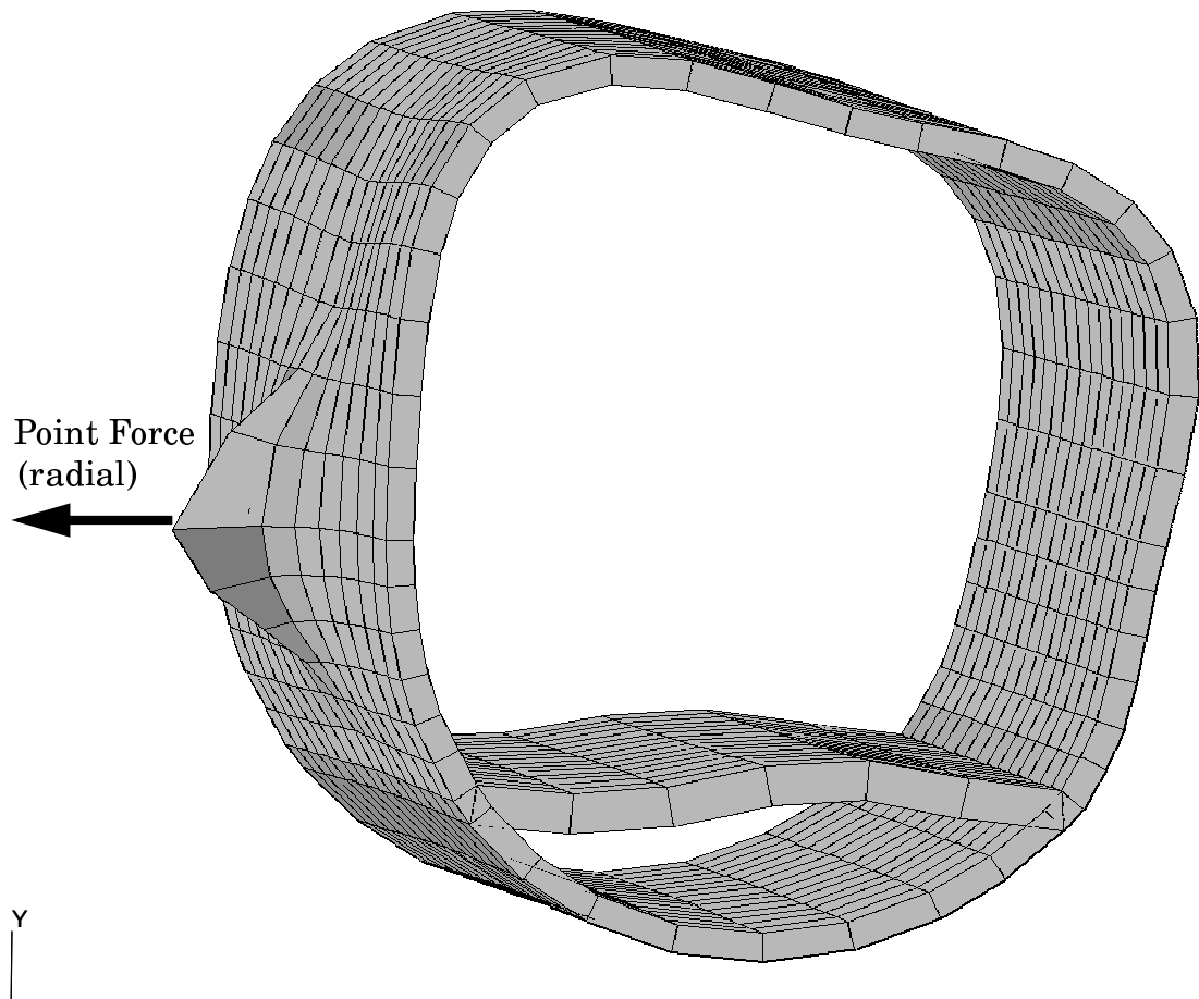
Figure 10: Response for a 82.0 Hz point force.
