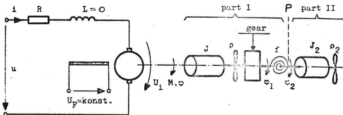
fig.2: electromechanical system representation
