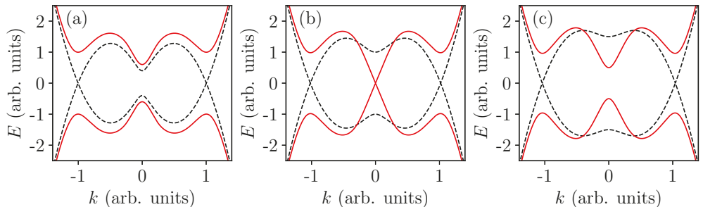
Figure 16: QP ( \Delta \neq 0 , red lines) and bare electron ( \Delta = 0 , black dashed lines) energy dispersion as a function of the momentum k for the MNW. (a) Trivial regime ( E_Z < 2\sqrt{\mu^2 + \Delta^2} ). (b) Topological transition ( E_Z = 2\sqrt{\mu^2 + \Delta^2} ). (c) Topological regime ( E_Z > 2\sqrt{\mu^2 + \Delta^2} ).
