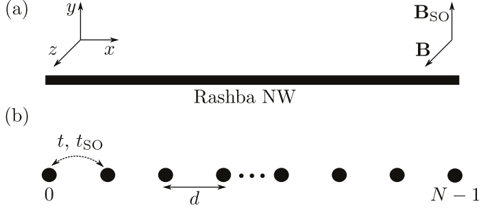
Figure 24: (a) Sketch of a Rashba NW subject to perpendicular magnetic and SO fields \mathbf{B} and \mathbf{B}_{\text{SO}} . (b) The discretized system consists of N sites and d is the lattice constant. The hopping amplitudes t and t_{\text{SO}} are also shown.
