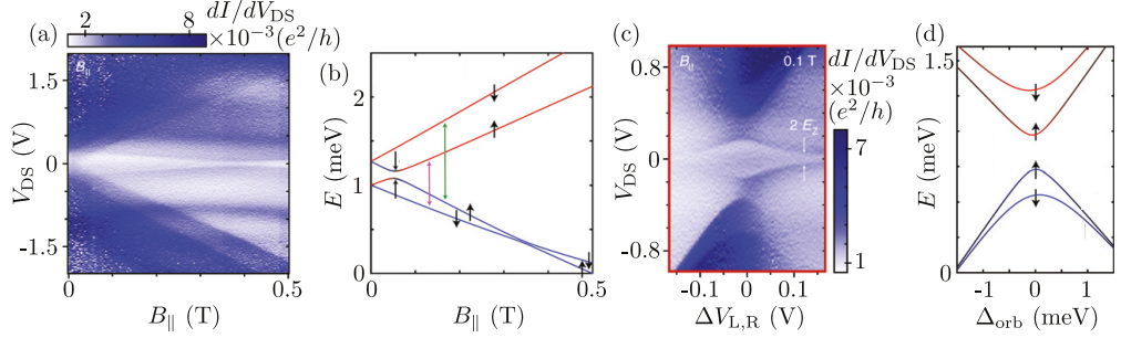
Figure 31: (a) Measured dI/dV_{DS} as a function of V_{DS} and B_{||} in the 1e regime of the (2,3) crossing. (b) Calculated energies of the states involved in the 1e regime of the (2,3) crossing as a function of B_{||} . The green and purple arrows denote the energies used to extract g -factors. (c) Measured dI/dV_{DS} as a function of V_{DS} and \Delta V_{L,R} in the 1e regime of the (2,3) crossing for B_{||} = 0.1 T. (d) Calculated energies of the states involved in the 1e regime of the (2,3) crossing as a function of \Delta V_{L,R} for B_{||} = 0.1 T. The figure is adapted from paper III.
