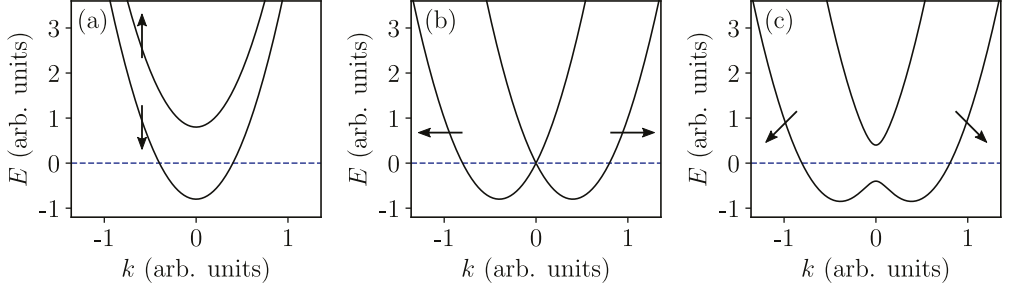
Figure 15: Dispersion relation of the bare NW for (a) E_Z \neq 0 , \alpha_{SO} = 0 , (b) E_Z = 0 , \alpha_{SO} \neq 0 , and (c) E_Z \neq 0 , \alpha_{SO} \neq 0 . The chemical potential is set to zero (dashed blue lines).
