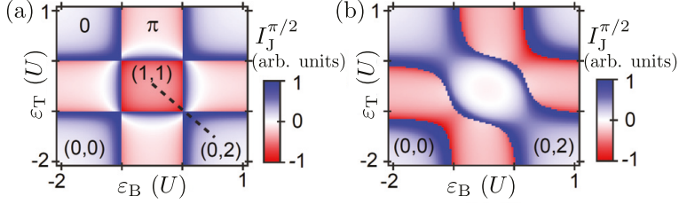
Figure 36: (a) Calculated I_J^{\pi/2} for the DQD Josephson junction as a function of the orbital energies \varepsilon_T and \varepsilon_B for a coupling t \approx 0 between the QDs. (b) As in (a) but for t = 0.2U . The figure is adapted from paper V.
