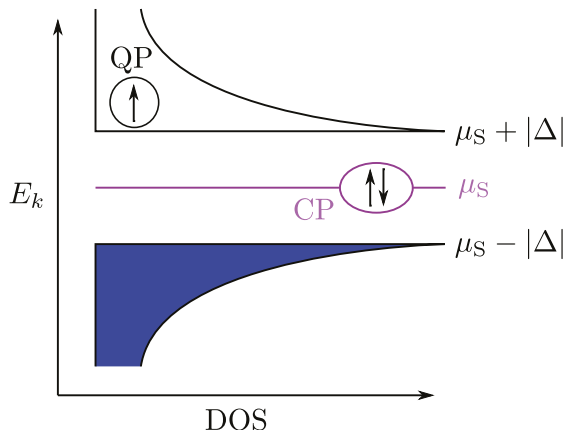
Figure 8: Sketch of the DOS with respect to energy E_k for QPs in a superconductor close to the Fermi level \mu_S . The blue (white) color denotes occupied (unoccupied) states. CPs (shown encircled by a purple ellipse) are at the Fermi level of the superconductor \mu_S (denoted with the purple line). In order to add a QP (spin in the black circle) to the superconductor, an energy |\Delta| must be paid with respect to \mu_S .
