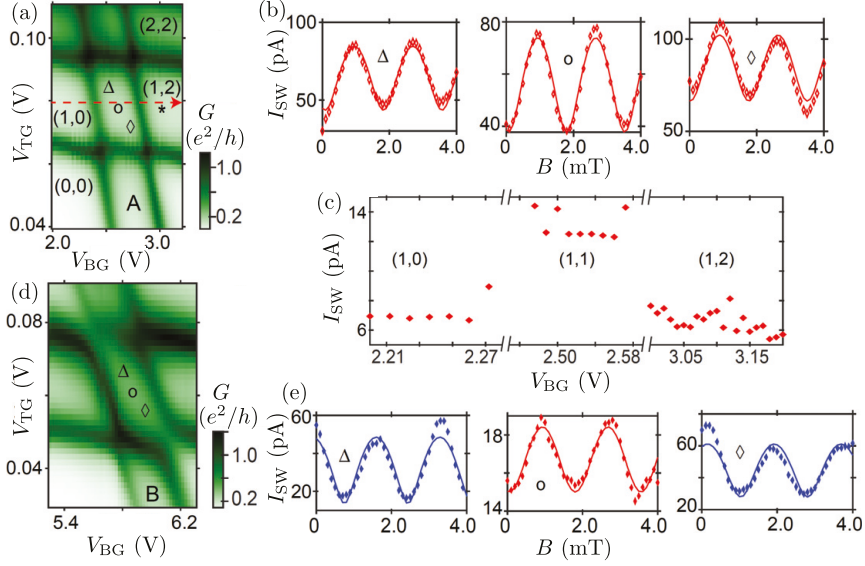
Figure 35: (a) Charge stability diagram for the weak-coupling crossing I. (b) I_{SW} as a function of B for the points in the (1,1) regime marked in (a). (c) I_{SW} for a varying V_{BG} along the red arrow shown in (a). (d) Charge stability diagram for the intermediate-coupling crossing II. (e) I_{SW} as a function of B for the points in the (1,1) regime marked in (d). In the panels corresponding to a \pi phase lines and points are plotted in red, while in the ones corresponding to a 0 phase they are plotted in blue. The figure is adapted from paper V.
