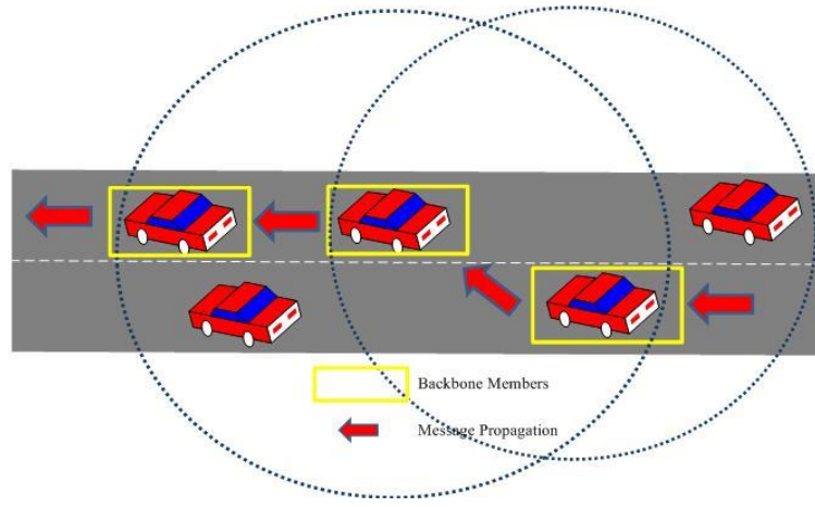
Fig.5. A backbone based scenario, the message have been rebroadcasted only by the backbone members
