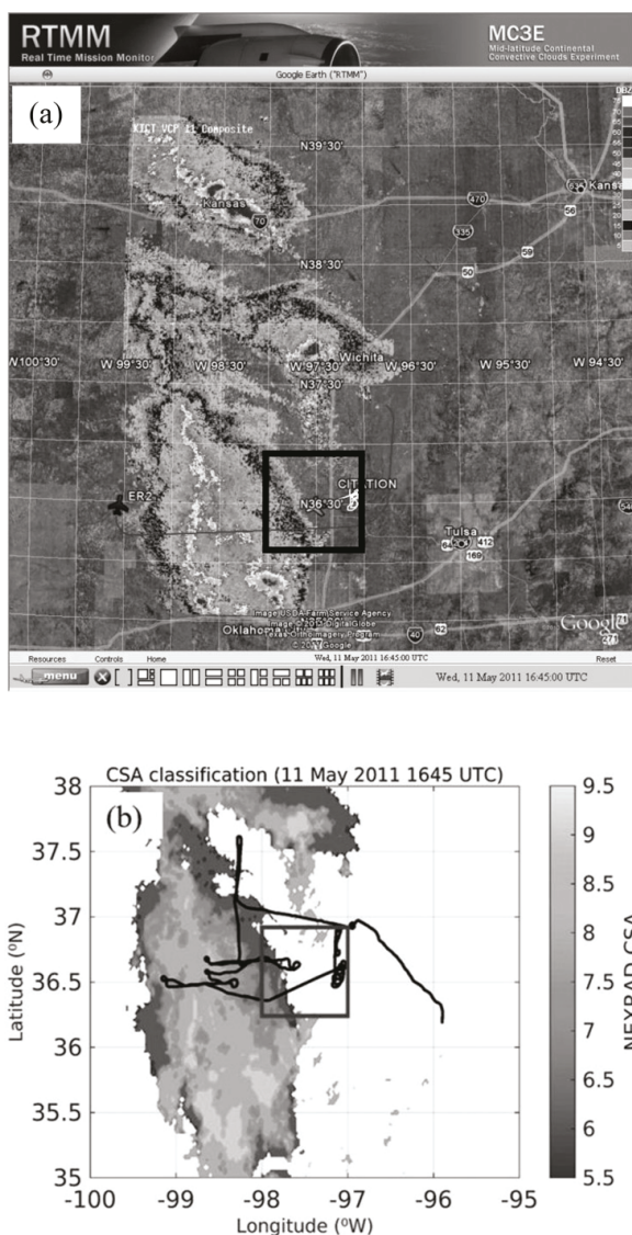
FIG. 2. (a) RTMM image during MC3E field campaign showing a plan position indicator of radar reflectivity from KICT radar at 1645 UTC with flight positions of citation (white line) and ER-2 aircraft (red line) (adapted from https://ghrc.nasa.gov/hydro ), (b) convective-stratiform-anvil (CSA)-classified deep convective systems and Citation aircraft flight track (plotted for the entire flight duration, black line) superimposed on it for the simulated day of the MC3E at 1645 UTC. The CSA classification is based on Feng et al. (2011) (thick anvil: 5.5–7.5; stratiform: 7.5–8.5; convective: 8.5–9.5). The black boxes in (a) and (b) indicate the simulation domain.
