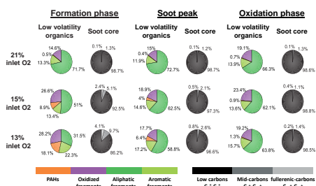
Figure 3: Soot chemical compositions during soot formation, soot peak and soot oxidation phases for 21%, 15% and 13% inlet O_2 concentrations. Left columns: grouped ion fragments originating
