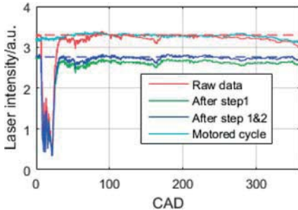
Figure 7. Transmitted laser signal compensation process
