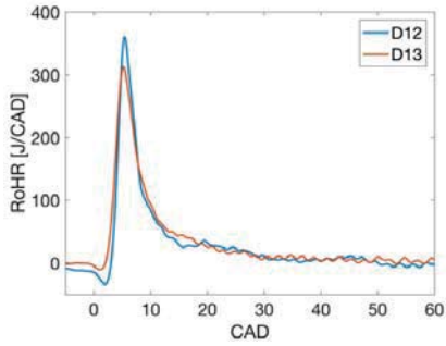
Figure 2b. Sample AHRR for the 15% [O 2 ] case.
