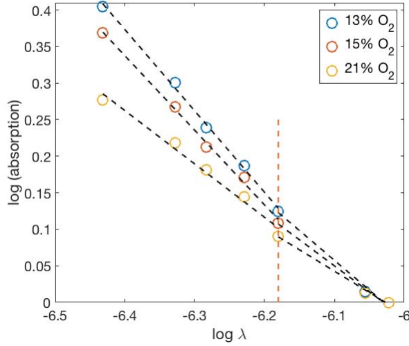
Figure 4.3 Log of absorption in function of the logarithm of the wavelengths for 13, 15 and 21% inlet oxygen at 50 CAD. The dashed black lines show the trends of the data. A break at the \log(660 \text{ nm}) is shown as an orange dashed line. The Ångström exponent corresponds to the slope of the trends.
