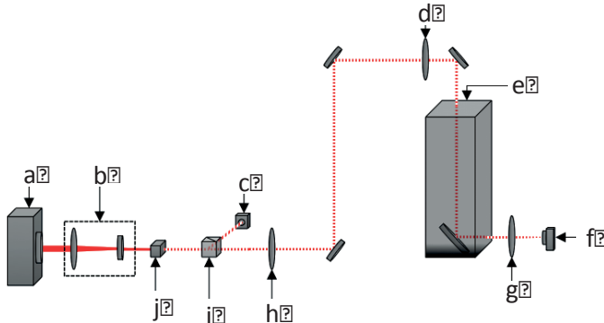
Figure 3. The parts of the laser extinction setup. Diode laser (a), telescope lenses (b), photodiode for the reference signal (c), re-collimation lens (d), schematic of engine (e), photodiode (f), collection lens (g), re-collimation lens (h), cubic beam splitter (i), and AOM (j).
