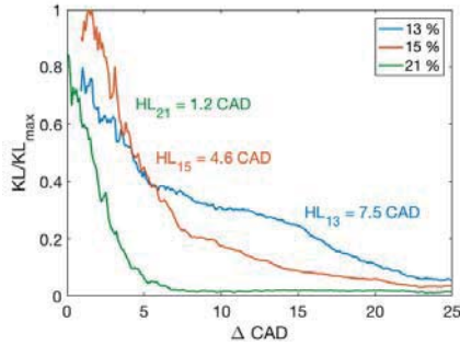
Figure 6a. Evolution of KL (relative to the peak KL at 15% O 2 ) in the optical measurements shown from the start of decay. The half-life extracted from the exponential approximation is shown in CAD.
