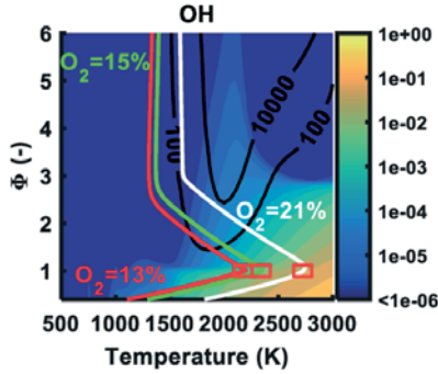
Figure 7. \Phi - T map of OH mass fraction constructed using a 0-D reactor with constant pressure, temperature and equivalence ratio. The three red squares highlight the maximum adiabatic flame temperature corresponding to the three cases (13, 15 and 21% O_2 ). The scale on the right represents the mass fraction of OH species.
