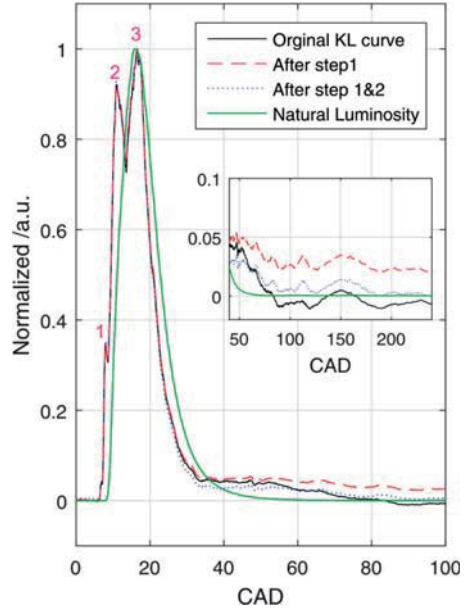
Figure 8. Normalized KL data and NL data.
