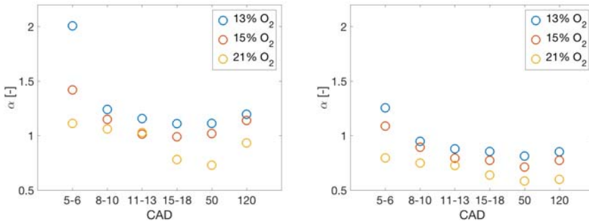
Figure 4.4 variation of the Ångström exponent during the cycle for varying inlet oxygen concentration. The left diagram shows the evolutions of Ångström exponent for shorter wavelengths (370-660 nm), on the right diagram are shown the evolutions for longer wavelengths (660-950 nm).
