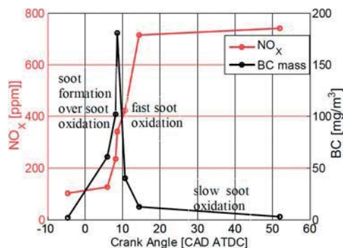
Figure 9. In-cylinder soot (Black Carbon) and \text{NO}_x concentration during combustion and expansion (0% EGR).
