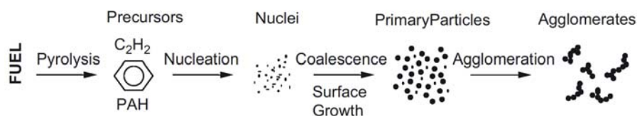
Figure 2.3 Soot particle formation process. Reproduced from [19].
