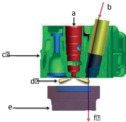
Figure 4. Section through the cylinder head used in the extinction setup. Injector location (a), laser entrance (b), cylinderhead (c), burning sprays (d), optical piston (e), and laser exit (f).
