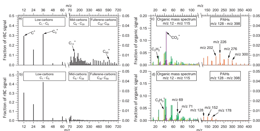
Figure 2: Refractory carbon cluster ion distributions and non-refractory organic ion fragments at 13% inlet O_2 concentration during intense soot formation (a and c) at 5 CAD (ATDC) and after intense soot oxidation (b and d) at 18 CAD (ATDC). Carbon clusters are divided into low-carbon clusters ( C_1^+-C_5^+ , left axis), mid-carbon clusters ( C_6^+-C_{29}^+ , right axis) and fullerenic-carbon clusters with even carbon numbers ( C_{30}^+-C_{58}^+ , right axis). Organic ion fragments: aliphatic fragments ( C_xH_{y>x}^+ , green), unsaturated and aromatic fragments ( C_xH_{y<x}^+ , light green), oxidized organic fragments ( C_xH_yO_z^+ , magenta) are shown on the left axis, and PAHs (orange) are shown on the right axis.
