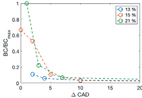
Figure 6b. Evolution of BC from the in-cylinder sampling measurements shown from the start of decay.
