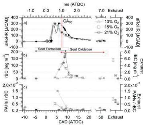
Figure 1: (a) In-cylinder heat release rates. Stars represent the start of combustion. The following symbols represent the aerosol sampling positions: triangles, 13% inlet O 2 ; squares, 15% inlet O 2 ; circles, 21% inlet O 2 . The CA50 was kept constant when changing EGR and is illustrated by the vertical red line. (b) SP-AMS rBC (soot) mass concentration. (c) The relative concentration of PAHs to rBC as a function of the combustion cycle. The position in the combustion cycle when particles were sampled with the FSV is shown in milliseconds (ms, top) and crank angle degrees (CAD, bottom) after the top dead center (ATDC, located at t=0). Three levels of EGR are shown corresponding to 21%, 15% and 13% O 2 inlet O 2 concentrations. Exhaust emission values are shown on the right axis. Black and red arrows show the soot formation dominated phase and soot oxidation dominated phase respectively. Error bars represent standard errors of the mean.
