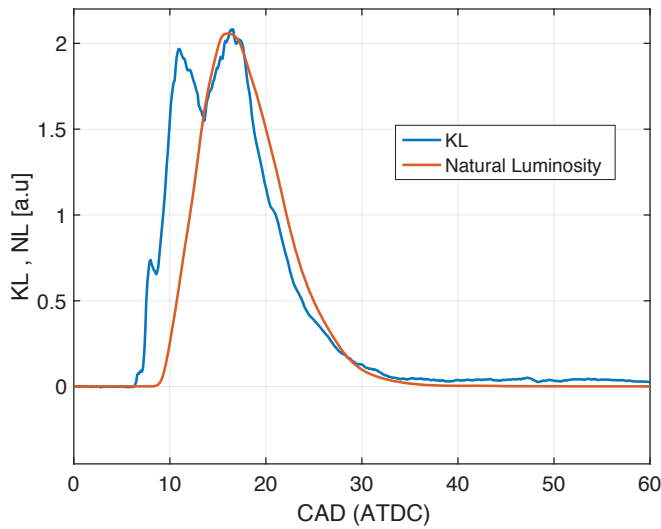
Figure 4.2 signals of LEM(KL) and NL during a combustion cycle.
