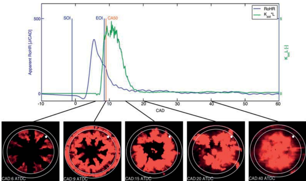
Figure 6. Images of natural luminosity of soot at different CAD related to the RoHR and the K_{ext} curve for 21% O_2 . The shutter speed is 0.25 \mu s until 15 CAD, 2.5 \mu s at 20 CAD and 20 \mu s at 40 CAD. The inner white circle represents the bowl wall, the outer one represents the periphery of the piston. The intensity is digitally rescaled through custom scaling color maps.
