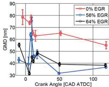
Figure 14. Geometric mean particle mobility diameter.
