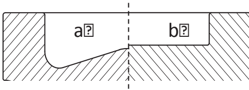
Figure 1. Profile of the metal piston used in the D13 engine (a) and of the quartz piston used in the D12 engine (b).
