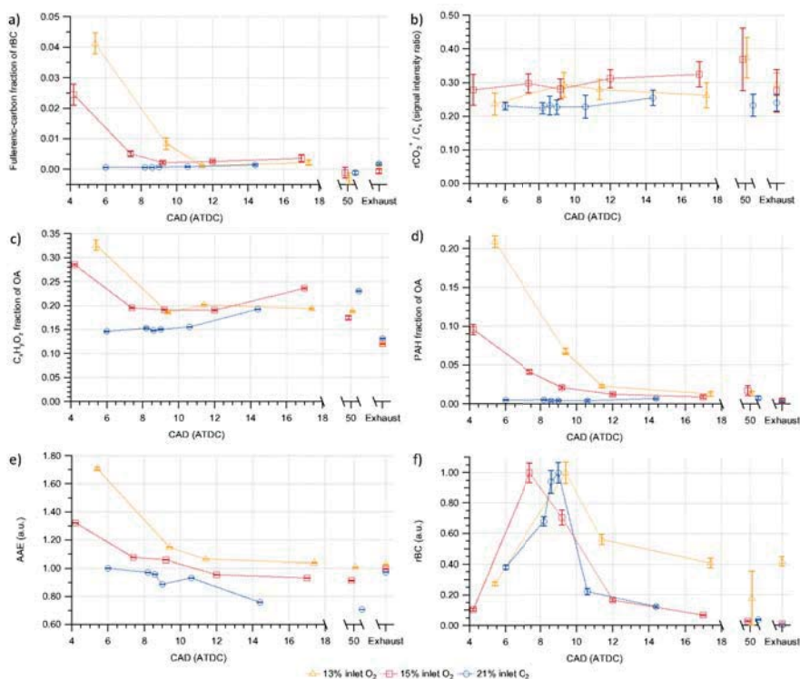
Figure 4: Evolution of soot properties during the combustion cycle and at 21%, 15% and 13% inlet O_2 concentrations. (a) Fullerene-carbon fraction of rBC. (b) rCO_2^+ normalized to the total refractory C_x^+ (i.e., carbon cluster, signal intensity). (c) Oxidized organic ( C_xH_yO_z^+ ) fraction of total OA concentration. (d) PAH fraction of total OA concentration. (e) Variations in AAE with
