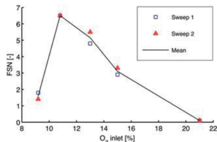
Figure 1. Measurements of Filtered Smoke Number (FSN) for a sweep in intake \text{O}_2 concentration. Soot emissions increase with reduction of intake \text{O}_2 , reach a maximum at 11% \text{O}_2 and then decrease again.
