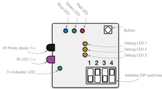
Figure 1. Shield layout
