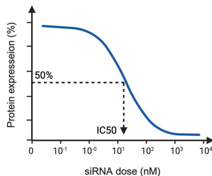
Figure 6. The dose-response relationship.
