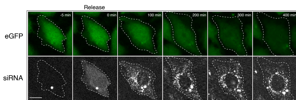
Figure 8. Cytosolic delivery of siRNA in eGFP expressing cell using confocal live-cell imaging.
