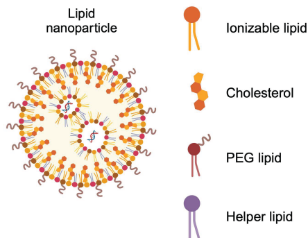
Figure 5. Lipid nanoparticle structure and composition.
