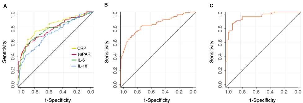
Figure 5. A) ROC curve for CRP (AUC: 0.80, 95% CI: 0.75-0.86), suPAR (AUC: 0.77, 95% CI: 0.71-0.83), IL-6 (AUC: 0.76, 95% CI: 0.71-0.82) and IL-18 (AUC: 0.71, 95% CI: 0.65-0.78) B) ROC curve for the combination of CRP and suPAR in all participants (AUC: 0.83, 95% CI: 0.78-0.88) C) ROC curve for the combination of CRP and suPAR in participants with CD4 count <200 cells/mm 3 (n=132, AUC: 0.93, 95% CI 0.89-0.97)
