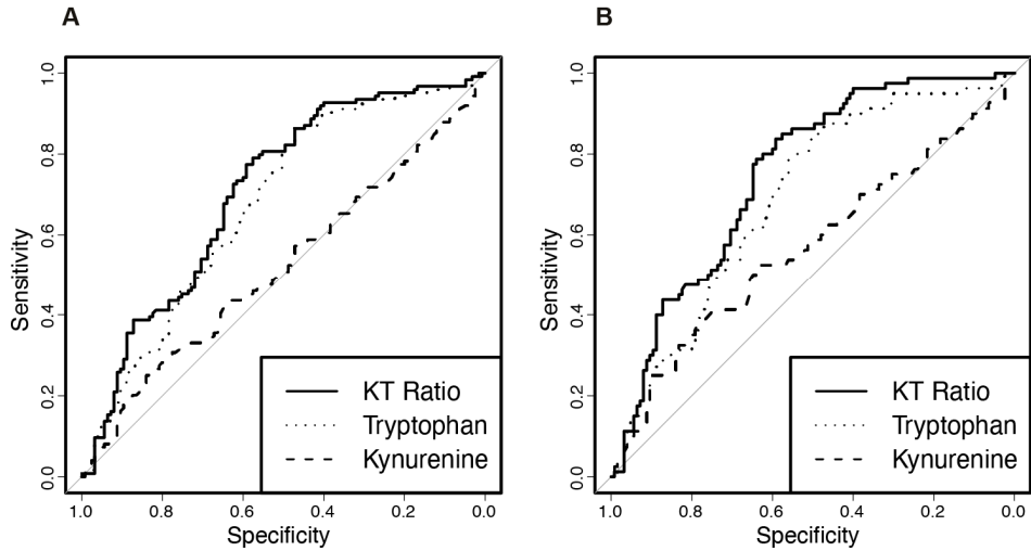
Figure 7. ROC curves for A) all participants. AUC for KT ratio: 0.70 (95% CI: 0.64-0.77), for tryptophan 0.67 (95% CI: 0.61-0.74 and for kynurenine 0.52 (95% CI: 0.45-0.59). B) Gene Xpert MTB/RIF and/or sputum smear positive participants (compared to HIV+/TB- participants) AUC for KT ratio 0.75 (95% CI: 0.68-0.81), for tryptophan 0.70 (95% CI: 0.62-0.76) and for kynurenine 0.56 (95% CI 0.48-0.65).
