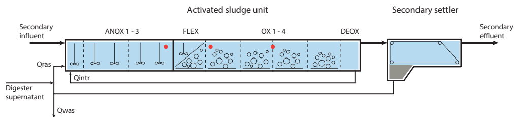
Figure 3.8: Schematic process configuration of the activated sludge reactors at Käppala wastewater treatment plant, Lidingö, Sweden. Red markers indicate positions for in-tank measurements of \text{N}_2\text{O} . Figure from Arnell et al. (2016b).
