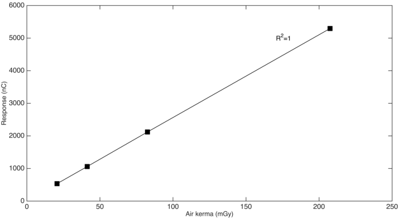
Figure 2. Response of the R100 detector versus air kerma for a 60 Co beam.
