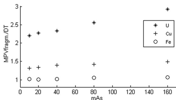
Figure 2. Graph shows the MPV_{frag}/DT quotient versus tube load for a fixed tube potential of 90 kVp for digital radiography and for fragment sizes in the range of 500–700 \mu m positioned on the right lung.
