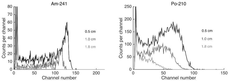
Figure 3. Pulse height distribution measured with the Si diode for a ^{241}\text{Am} source ( E_\alpha = 5486 and 5443 keV) (left) and a ^{210}\text{Po} ( E_\alpha = 5304 keV) (right) at three different distances: 0.5 , 1.0 , and 1.8 cm.
