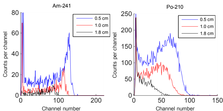
Figure 8 Pulse height distribution measured with the Si CT dose profiler (CTDP) for an electrodeposited ^{241}\text{Am} source ( E_\alpha = 5486 and 5443 keV) (left) and an encapsulated ^{210}\text{Po} source ( E_\alpha = 5304 keV) (right) at various SDD (0.5, 1.0, and 1.8 cm).
