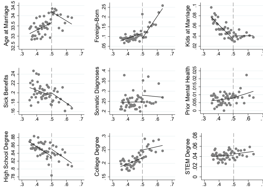
Figure B.2: Balancing by Control Variables
