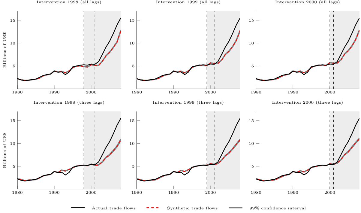
Figure 6. Average actual and synthetic bilateral trade flow between Denmark and Sweden using alternative intervention years.
