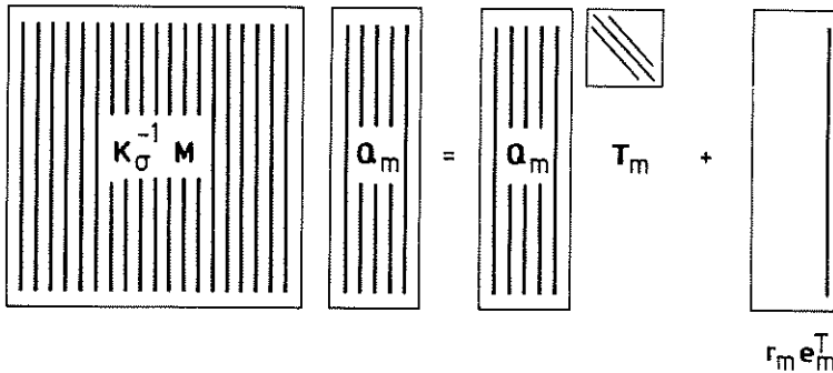
Fig. 4.1 The matrix form of the three-term recurrence formula for the generalized symmetric definite problem.
