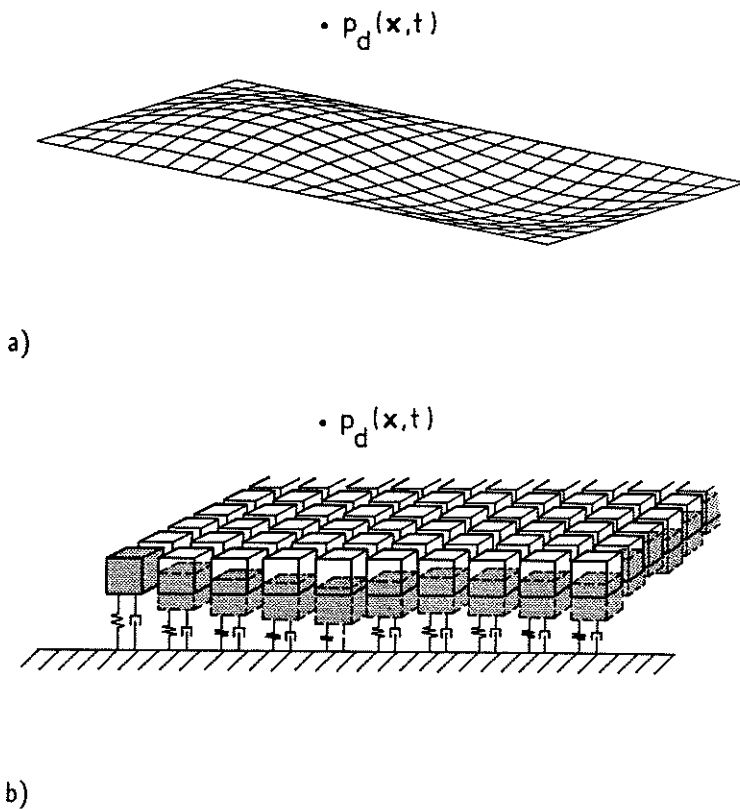
Fig. 3.1 Structural members subjected to a dynamic fluid pressure field p_d(x, t) . a) Continuous structure illustrated by a vibrating plate. b) Locally reacting surface modelled as a set of individual single degree-of-freedom systems.
