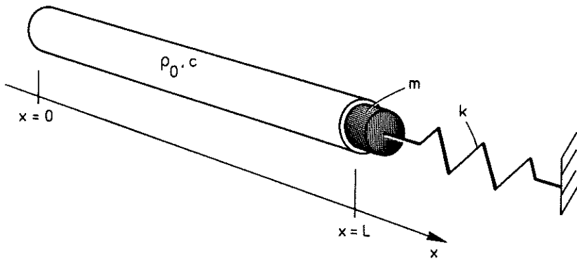
Fig. 5.1 Rigid wall cylinder filled with water and with a spring supported piston. c = 1500 \text{ m/s} , \rho_0 = 1000 \text{ kg/m}^3 , L = 3 \text{ m} , A = 1 \text{ m}^2 , m = 200 \text{ kg} , k = 493.48 \text{ MN/m}
