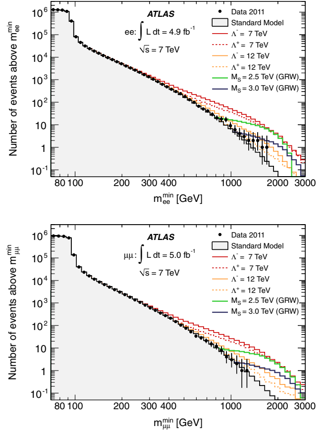
FIG. 3 (color online). Distribution of the number of events with dilepton mass above m_{\ell\ell}^{\min} for data (points) and SM prediction from Monte Carlo simulation (filled histograms, shaded gray) in the dielectron channel (top panel) and dimuon channel (bottom panel). The open solid and dashed histograms correspond to the expected distributions in the presence of contact interactions or large extra dimensions for several model parameters. The bin width is constant in \log(m_{\ell\ell}^{\min}) .
