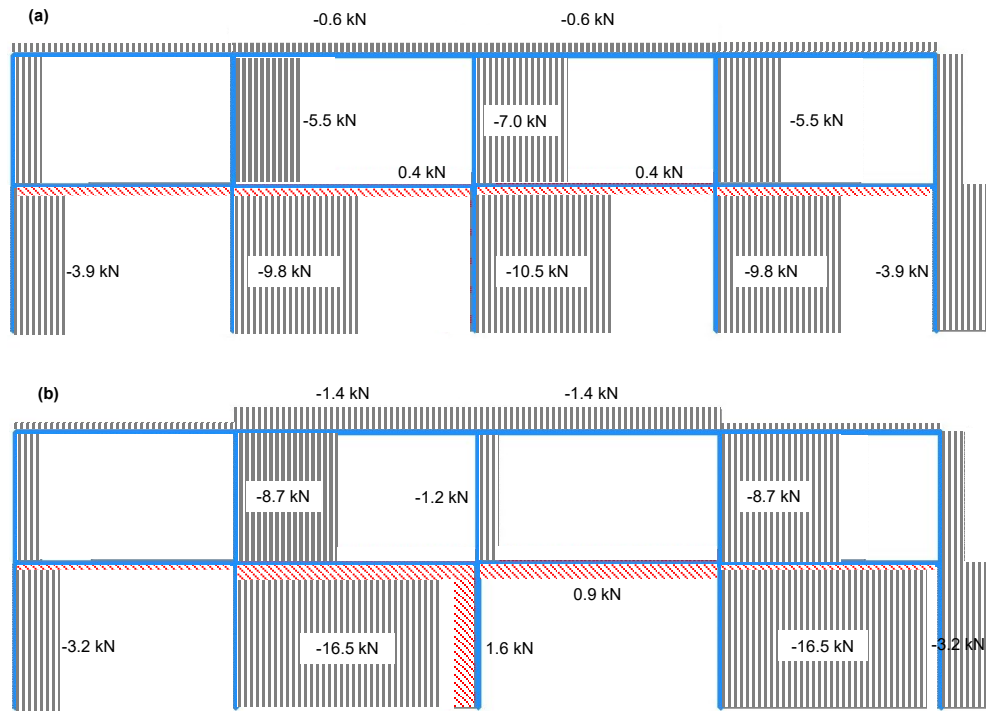
Fig 23. Axial forces in the frame members (a) before the fire and (b) at the end of the fire. Compressive forces are negative.
