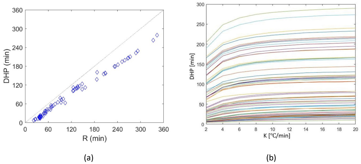
Fig 7a-b. Results from a numerical study on the DHP of 74 reinforced concrete columns. (a) Relationship between R and DHP using the cooling rate from EN1991-1-2 (Gernay, 2019). (b) DHP as a function of cooling rate K (Gernay et al., 2023b).
