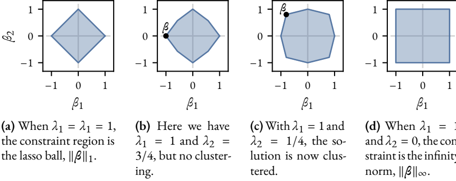
Figure 8: SLOPE balls (the sorted \ell_1 norm) for various choices of the penalization weight vector \lambda . It is the kinks at the boundaries, occurring when |\beta_1| = |\beta_2| , that induce clustering. The larger the difference between adjacent values in \lambda , the stronger the clustering effect becomes.
