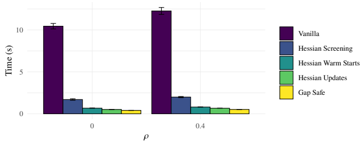
Figure 7: Incremental contribution to the decrease in running time from Hessian screening, Hessian warm starts, our effective updates of the Hessian and its inverse, and gap safe screening. In other words, Gap Safe , for instance, includes all of the other features, whilst Hessian Warm Starts includes only Hessian Screening . Vanilla does not include any screening and only uses standard warm starts (from the solution at the previous step along the path). The example shows an example of ordinary (least-squares) lasso fit to a design with n = 200 and p = 20\,000 with pairwise correlation between predictors given by \rho . (See Section 4 for more details on the setup). The error bars indicate standard 95% confidence intervals. The results are based on 10 iterations for each condition.
