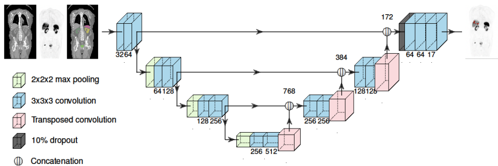
Figure 17. Illustration of the UNet3D architecture
