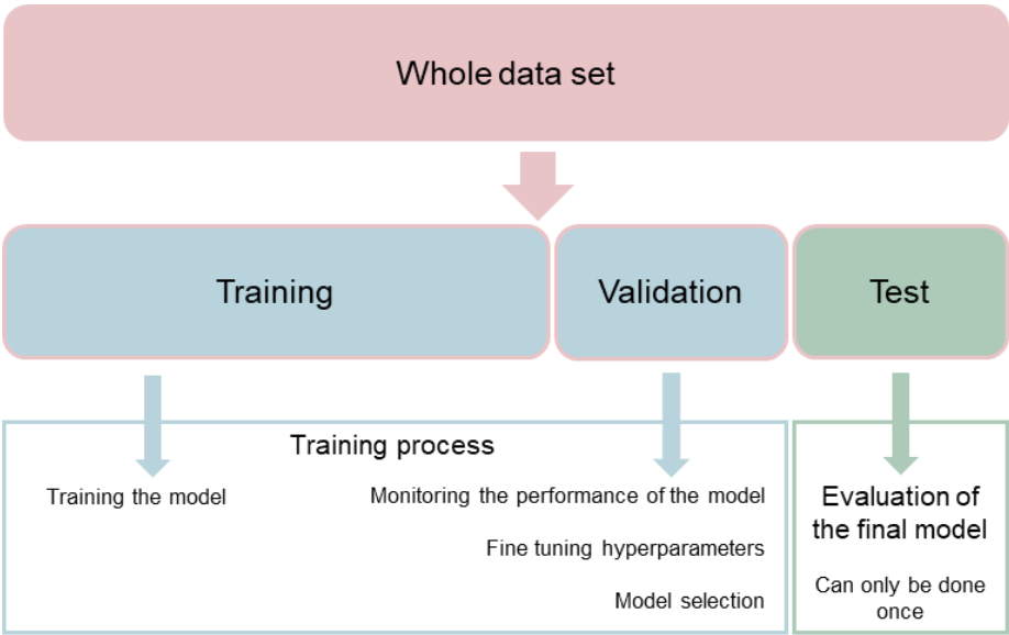
Figure 15. Dataset partitioning Image illustrating the partitioning of the entire data set into training, validation and test sets. Image adapted from the original by Yamashita et al. 178 Convolutional neural networks: an overview and application in radiology. Insights in imaging 9, 2018. Distributed under CC BY 4.0; https://creativecommons.org/licenses/by/4.0/
