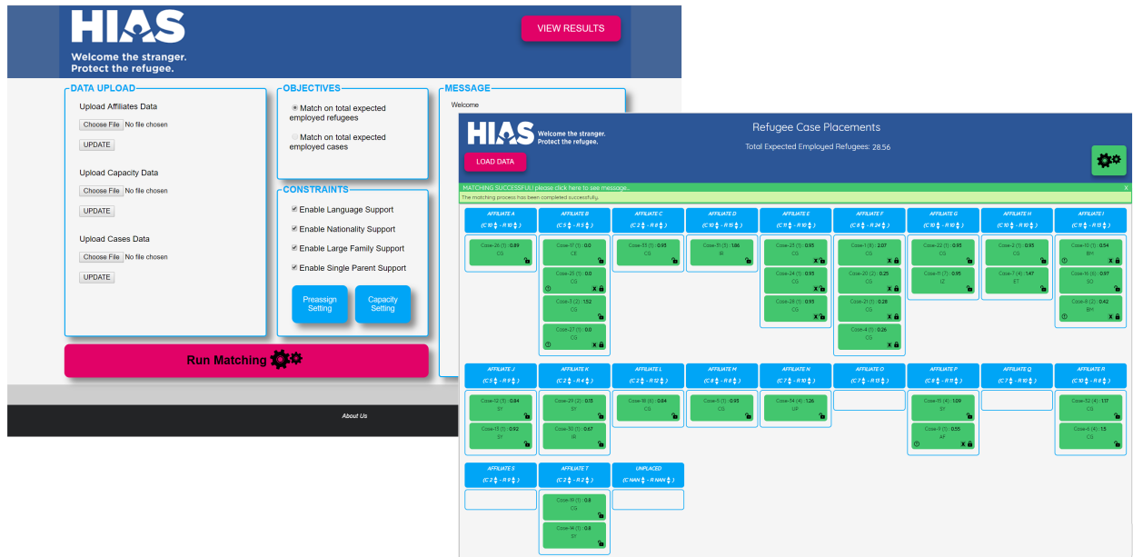
Figure 6: Annie Interface.
