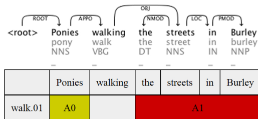
Figure 2: A representation of a parsed sentence: The upper part shows the syntactic dependency graph and the lower part shows the predicate, walk , and its two arguments the parser has extracted: Ponies and the streets in Burley .
