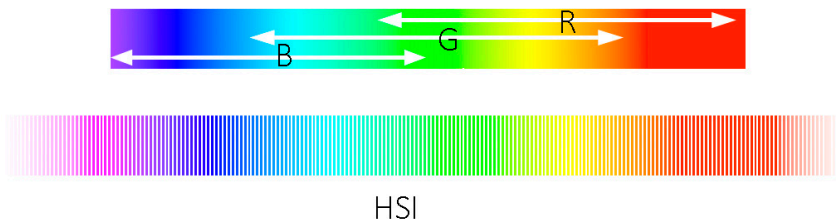
Figure 8. Spectral bands.
