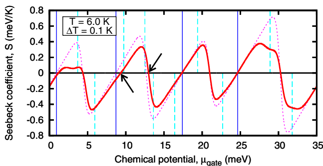
FIG. 4. Thermopower at T = 6.0 K, \Delta T = 0.1 K. The effect of excited states (vertical cyan dashed) on the thermopower lineshape (red thick solid) is smeared out due to temperature broadening. Still, the thermopower appears skewed and its zeroes are even shifted (arrows) off their usual positions, i.e., at the Coulomb peak positions (vertical blue solid) and in the middle of those. Shown as a reference, by excluding the excitations, the thermopower has the well known saw-tooth shape (magenta dotted).
