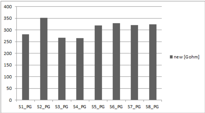
Fig. 7.14 Measured insulation resistance [ G\Omega ] between 2 randomly grouped strands for multiple motorette specimens before thermal cycle #1 applied
