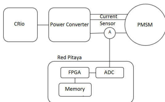
Fig. 6.16 Block diagram of the off-line on-board test set-up
