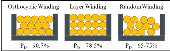
Fig. 3.5 Winding configurations [51]
