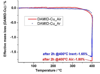
(b) Effective mass loss [%] after 2 hours of isothermal stage
