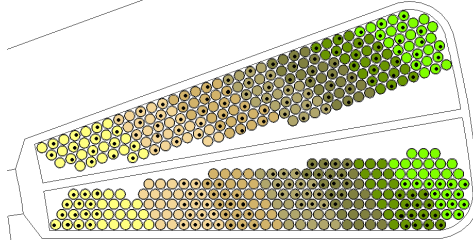
Fig. 3.3 7-turn 29-strand conductor distribution inside the slot by considering the ideal packing between the wires. The groupings of parallel strands are distributed in the upper half and concentrated in the lower half. [47]
