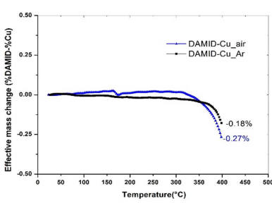
(a) Effective mass loss [%] before 2 hours of isothermal stage
