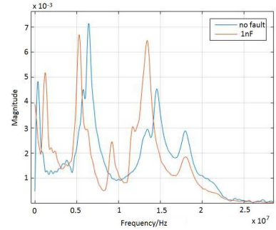
(b) Current responses (absolute value) in frequency domain
