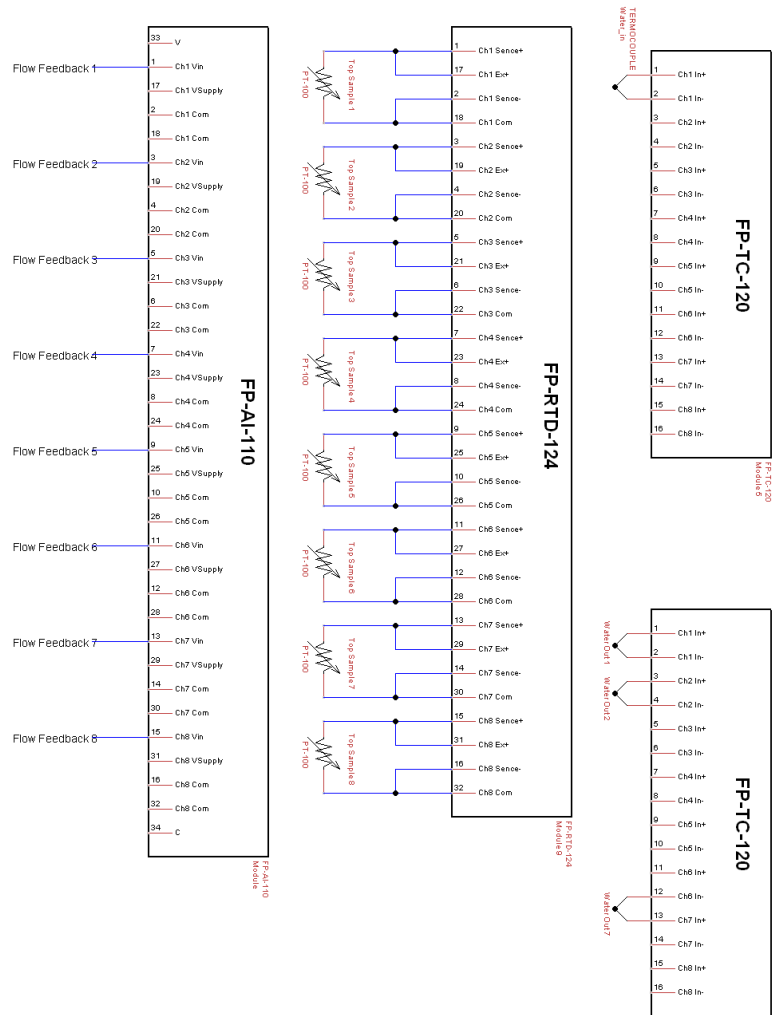
Fig. A.1 Control schematics for accelerated aging test - logging of flow rates, temperatures of motorette iron and coolant
