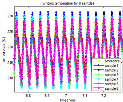
Fig. B.1 Measured hot spot temperature in windings of the 6 motorette specimens in accelerated test (thermal cycle #1, defined in Table 7.2)
