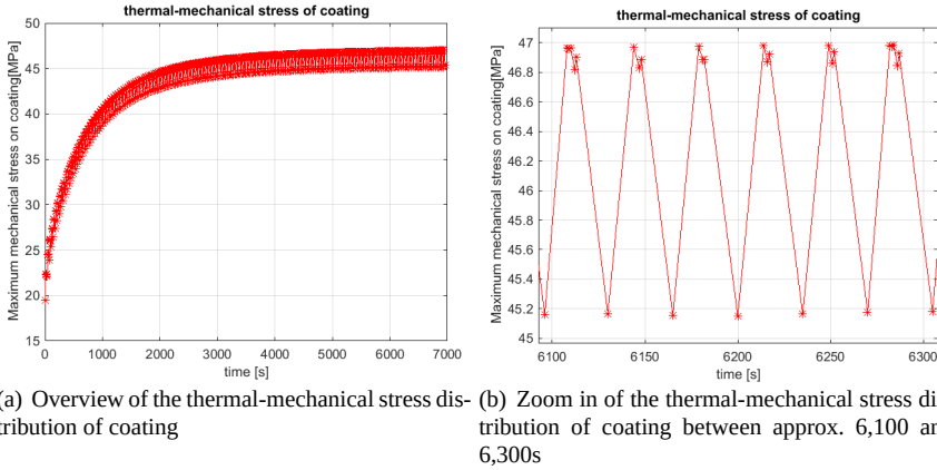
Figure 7.32: Mechanical stress of coating induced by thermal stress of the VCE machine stator after running 200 times of SLC
