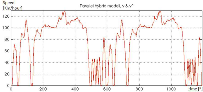
Fig. 5.3 US06 driving cycle
