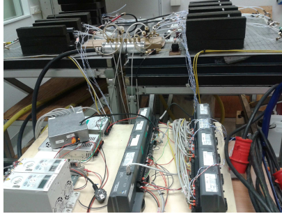
(a) Test rig built for accelerated tests - view 1 (including control hardware)
