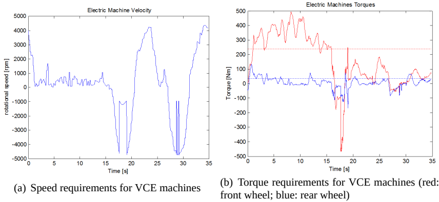
Figure 7.28: Speed and torque requirements for VCE electrical machines
