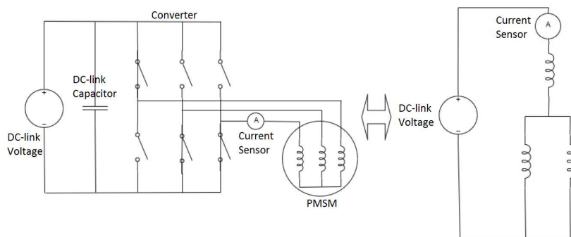
Fig. 6.15 Equivalent circuit of electrical machine when a voltage pulse is generated by drives
