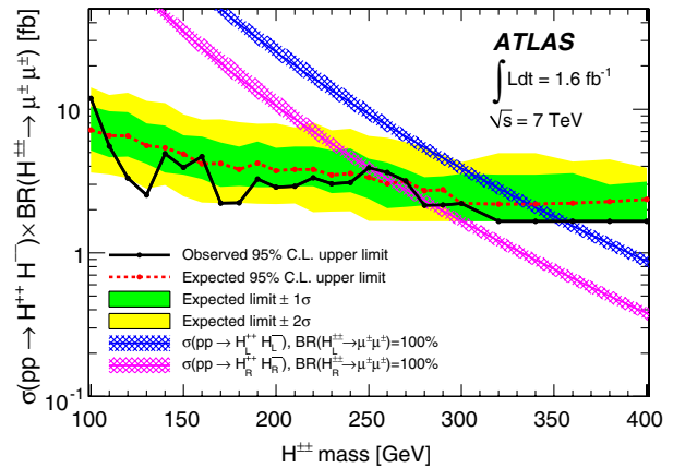
FIG. 2 (color online). Upper limit at 95% C.L. on the cross section times branching ratio for pair production of doubly charged Higgs bosons decaying to two muons. Superimposed is the predicted cross section for H_L^{++} H_L^{--} and H_R^{++} H_R^{--} production assuming a branching ratio to muons of 100%. The bands on the predicted cross sections corresponds to the theoretical uncertainty of 10%.
