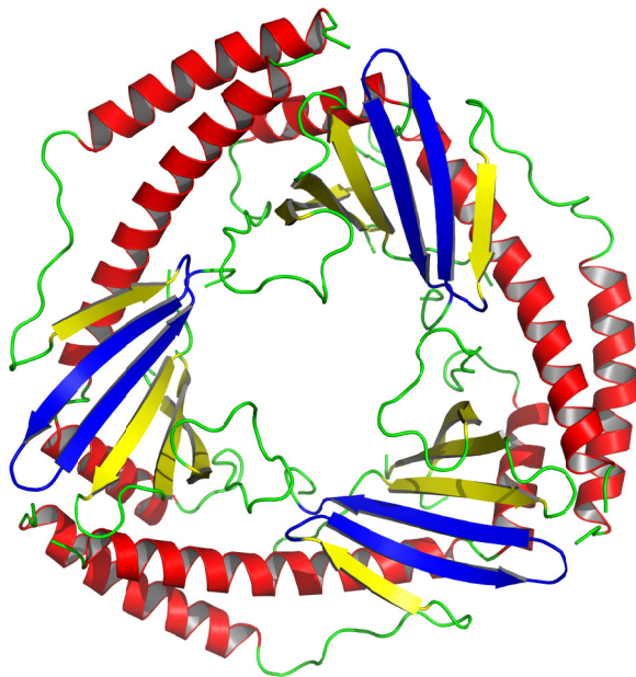
Figure 9. Structure of p33. Trimeric conformation of p33 drawn as a cartoon diagram. Blue area in each of the subunits represents the proposed LL-37 binding domain (aa 115-135). Figure created using the crystal structure by Jiang et al. [291], downloaded from RCSB PDB.
