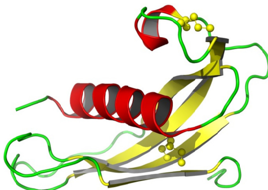
Figure 1. Structure of hCLD. Drawn as a cartoon diagram, yellow spheres indicates the two disulfide bonds. Figure created using PyMOL and the crystal structure obtained by Pazgier et al. [23], downloaded from RCSB PDB.
