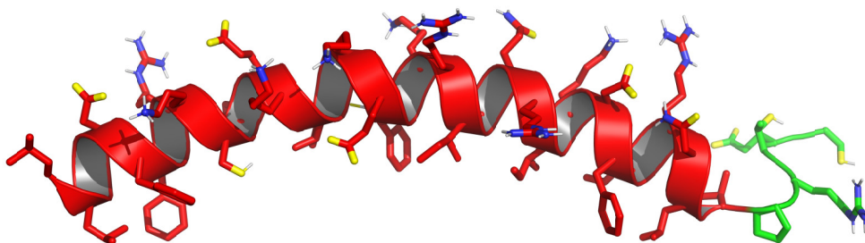
Figure 2. Structure of LL-37. Drawn as a cartoon diagram with sticks indicating amino acid side chains, nitrogen as blue, oxygen as yellow, polar hydrogens as white. Secondary structure is shown as elucidated by Wang et al. [34] using NMR spectroscopy of LL-37 in solution complex bound to deuterated SDS micelles. The structure is highly affected by environmental factors. Here, it consists of one \alpha -helix covering residue 2-31 followed by disordered C-terminal residues.
