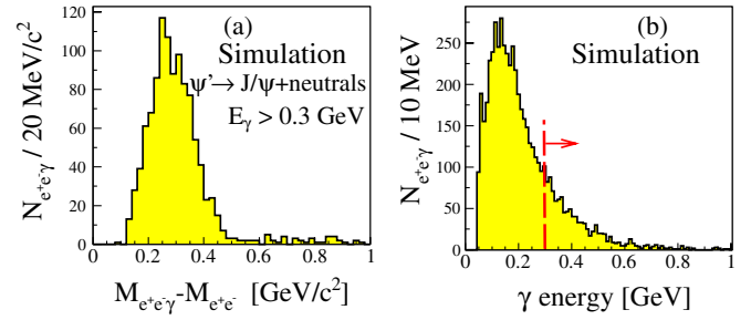
FIG. 15 (color online). Mass (a) and \gamma energy (b) distributions of \psi' \rightarrow J/\psi + \text{neutrals} \rightarrow e^+e^-\gamma obtained from simulations. The dashed line in panel (b) represents the photon energy cut applied in this analysis. Appropriate scaling indicates that such events contribute between 6 and 20 counts to the correlated e^+e^-\gamma distribution.
