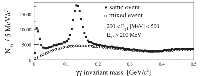
FIG. 10. \gamma\gamma mass distribution in the \pi^0 region used to study \gamma detection resolution. One photon is required to have energy between 200 MeV and 500 MeV, while the other is required to have energy greater than 200 MeV.
