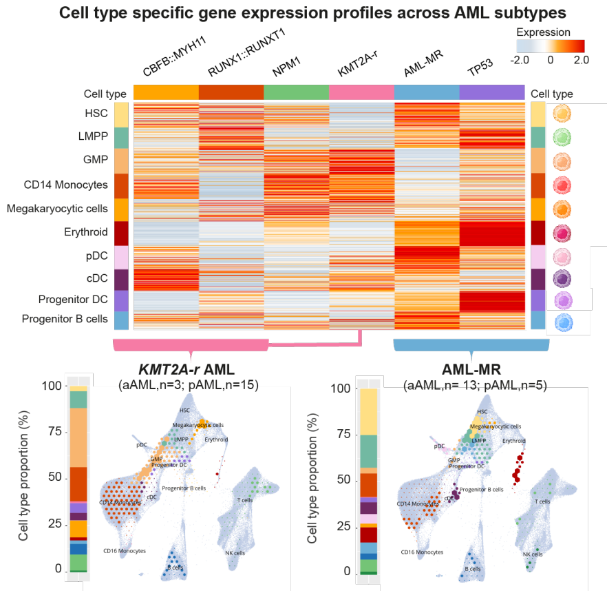
Figure AIV-1 | The maturation characteristics of AML. Heatmap showing cell type-specific gene expression across various AML genetic subtypes, with red indicating high expression (upper). Cell composition is visualized by bar plots, and maturation characteristics are displayed in single-cell projections of AML cells onto a normal bone marrow reference for KMT2A-r AML (lower left) and AML-MR (lower right).
