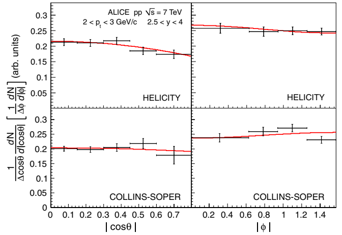
FIG. 2 (color online). The acceptance-corrected angular distributions for the J/\psi decay muons, for 2 < p_t < 3 GeV/c. The simultaneous fit to the results in the CS and HE frames is also shown. The plotted errors are purely statistical. The horizontal bars represent the bin width.
