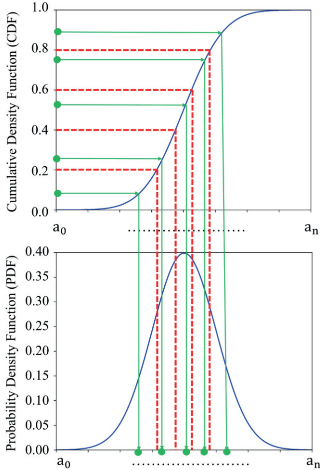
Figure 7: Latin hypercube sampling (LHS).
