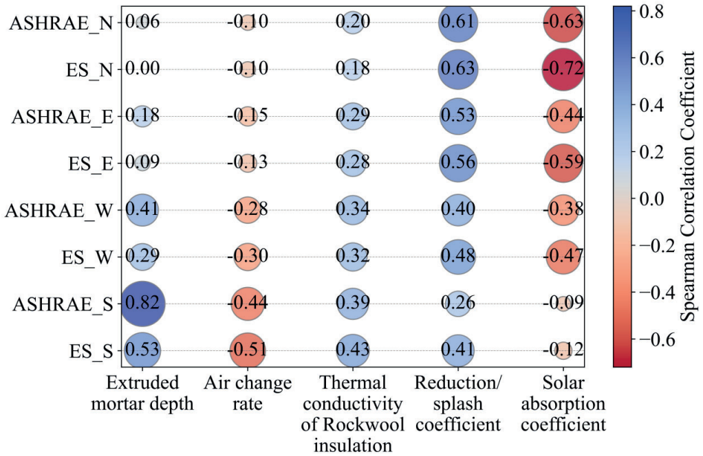
Figure 9: Spearman correlation coefficients between the input variables and maximum mould index (MMI). Colourmap guide: 0.00-0.09: negligible relationship, 0.10-0.39: weak relationship, 0.40-0.69: moderate relationship, 0.70-0.89: strong relationship, 0.90-1.00: very strong relationship.
