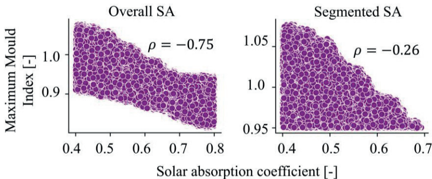
Figure 17: Overall vs segmented sensitivity analysis according to MSA method.
