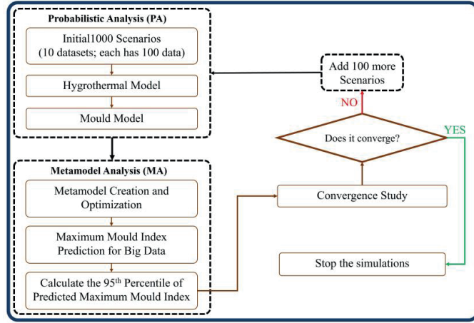
Figure 1: Probabilistic mould growth analysis procedure.
