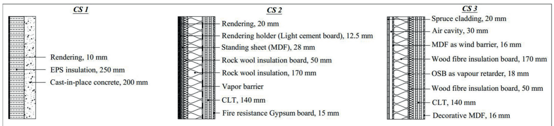
Fig. 3. Three external wall assemblies, case studies 1 and 2 adopted from [77].
