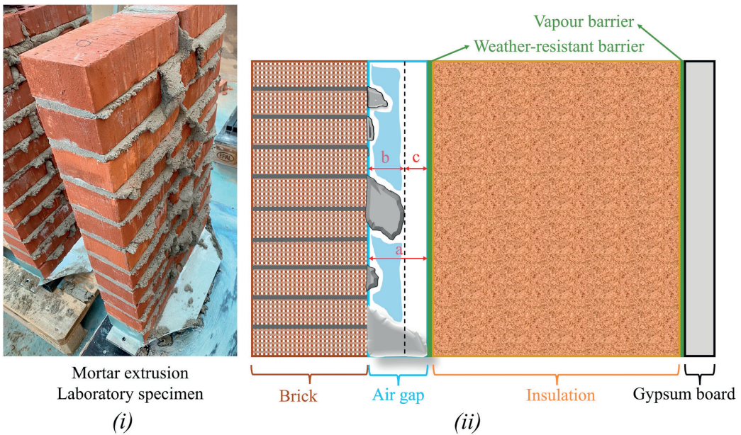
Fig. 4. Mortar extrusion phenomenon for clay brick cladding (the dimensions are not scaled). a [mm]: whole air cavity thickness, b [mm]: extruded mortar thickness, c [mm]: net air cavity thickness. Grey clouds: extruded mortar. Blue clouds: existing air between extruded mortar.
