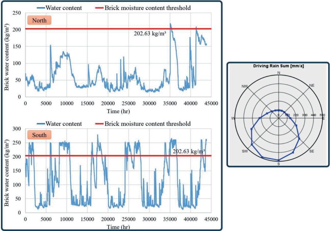
Figure 8: Water content of clay brick masonry façade (left side) between 2018 and 2023 where the red line is the brick moisture content threshold based on ES water penetration criterion, WDR chart (right side).
