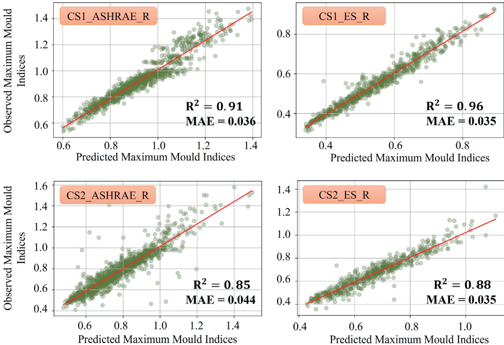
Fig. 8. Predicted vs observed data during the machine learning model testing, Rensjön (R). ES: case studies (CS1 and CS2) based on experimental study data.
