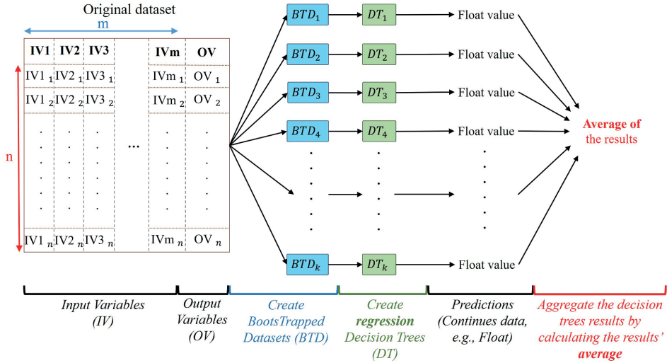
Fig. 2. Overview of the regression Random Forests (RF).
