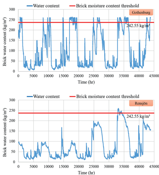
Fig. 11. Water content of clay brick masonry façade in Gothenburg (top) and Rensjön (bottom) between 2018 and 2023.
