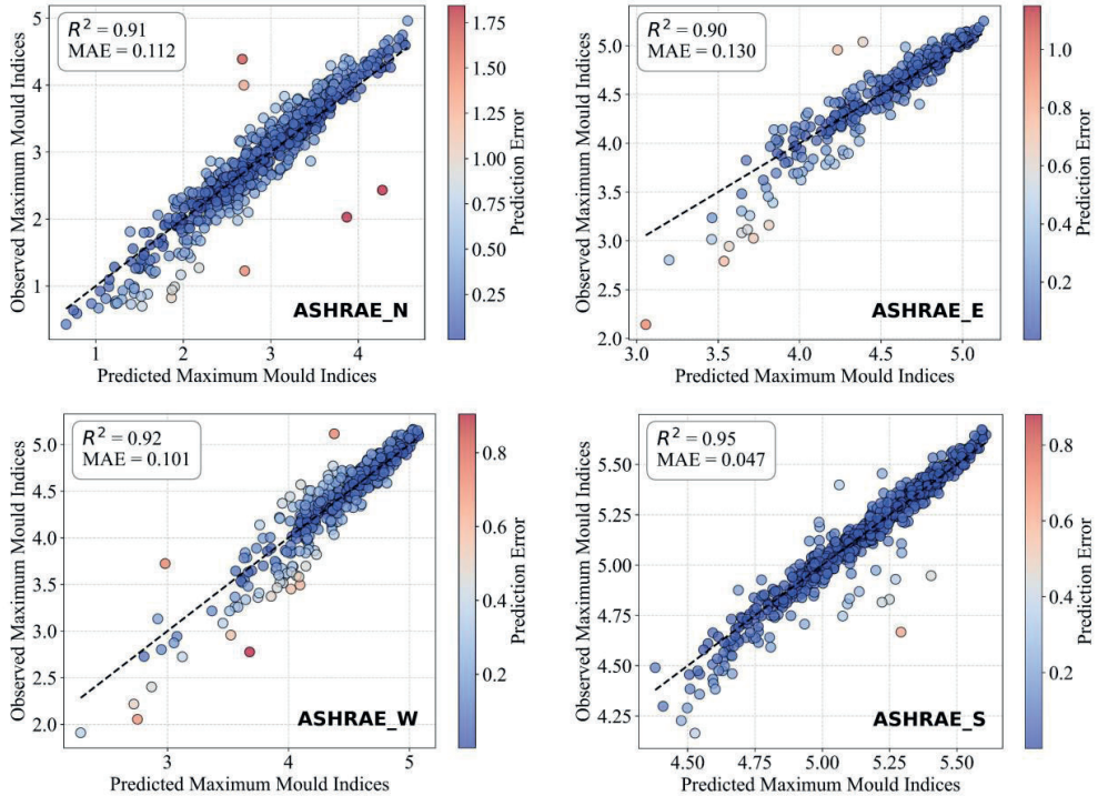
Figure 6: Predicted vs observed data during the machine learning model testing, using ASHRAE standard. N: north, E: east, W: west, S: south.
