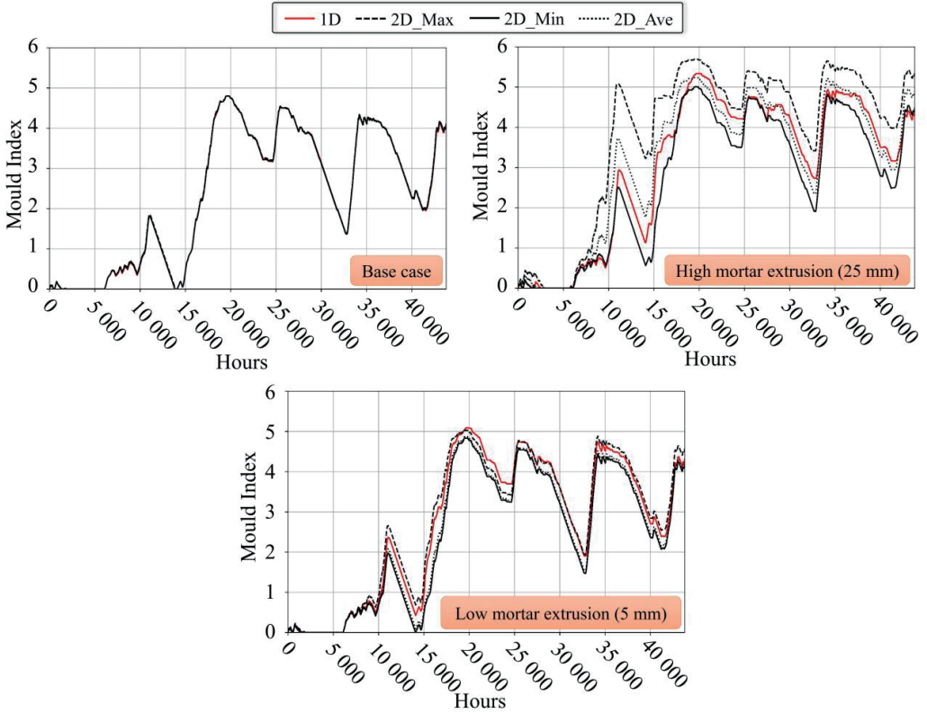
Figure 5: Wall assemblies modelling for verification, 1D versus 2D. Max/Min/Ave: maximum/minimum/average mould index [-] within the 1 m height of the wall in the 2D model.
