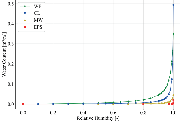
Fig. 3. Sorption isotherms of four different insulations [23]. WF: wood fibre, CL: cellulose, MW: mineral wool, and EPS: expanded polystyrene.
