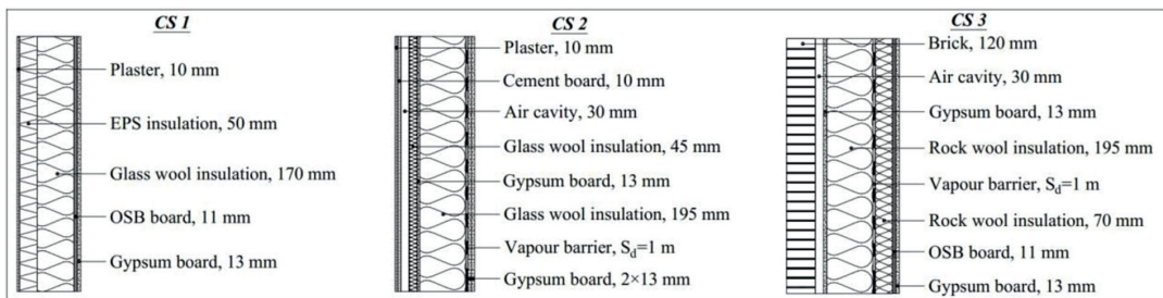
Fig. 2. Three external wall assemblies: case study 1 (CS1), case study 2 (CS2), and case study 3 (CS3).
