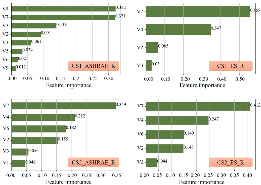
Fig. 10. Feature importance analysis, Rensjön (R). ES: case studies based on experimental study data. V1: extruded mortar depth; V2: air change rate; V3: thermal conductivity of Rockwool insulation; V4: reduction/splash coefficient; V5: outdoor convection heat exchange coefficient; V6: saturation point of brick; V7: solar absorption coefficient; V9: long-wave emissivity.
