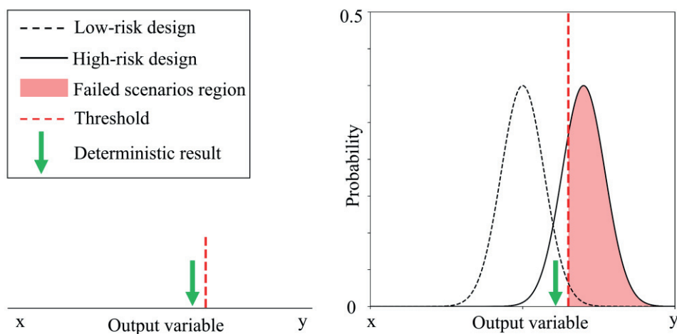
Figure 5: Visualisation of deterministic (left) and probabilistic (right) analyses. The red dashed line indicates the performance threshold, with values to the left considered acceptable. For clarity, probability values exceeding 0.5 on the y-axis have been omitted from the visualisation.
