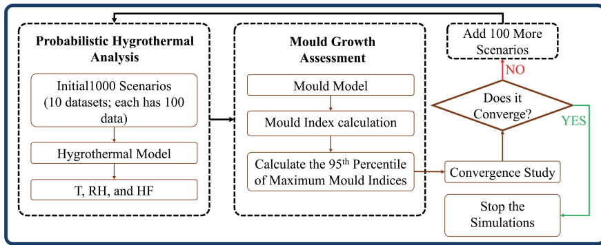
Fig. 1. Probabilistic hygrothermal and mould growth analyses procedure. T: temperature, RH: relative humidity, and HF: heat flux.
