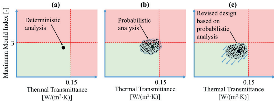
Figure 6: Probabilistic analysis (PA) application in hygrothermal analysis.
