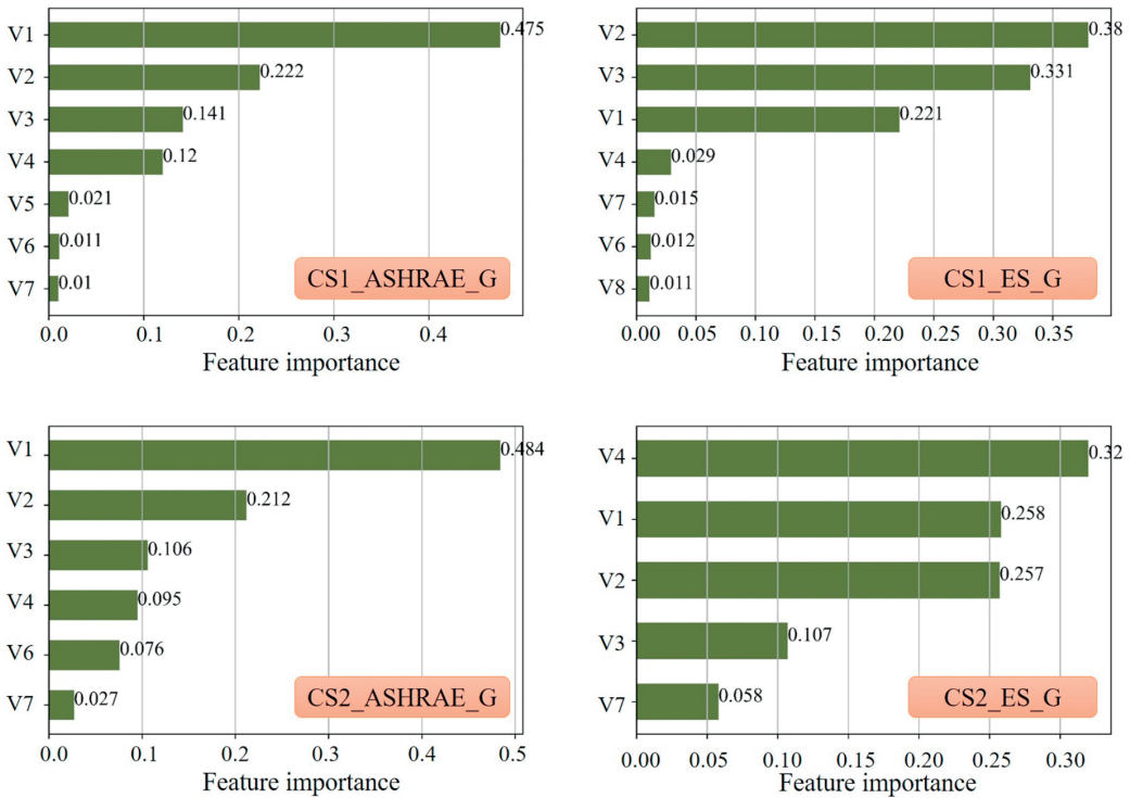
Fig. 9. Feature importance analysis, Gothenburg (G). ES: case studies based on experimental study data. V1: extruded mortar depth; V2: air change rate; V3: thermal conductivity of Rockwool insulation; V4: reduction/splash coefficient; V5: outdoor convection heat exchange coefficient; V6: saturation point of brick; V7: solar absorption coefficient; V8: thermal conductivity of brick.
