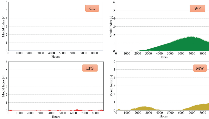
Fig. 4. Mould growth assessment [-]. CL: cellulose, WF: wood fibre, EPS: expanded polystyrene, and MW: mineral wool.
