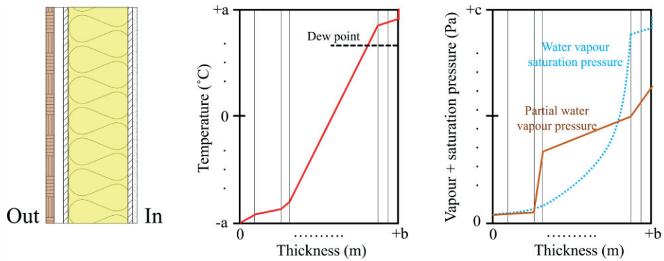
Figure 2: Left : Timber frame wall, Middle : dew point vs temperature, Right : partial water vapour pressure vs water vapour saturation pressure. Intersections mean interstitial condensation.
