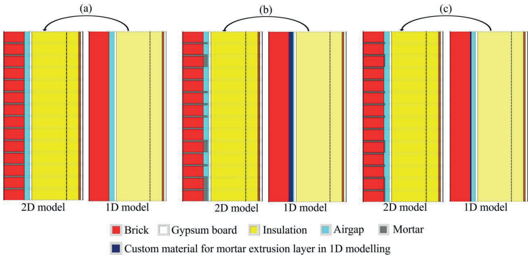
Figure 4: 1D versus 2D modelling for hygrothermal model verification. (a) base case, (b) high mortar extrusion (25 mm), and (c) low mortar extrusion (5 mm).
