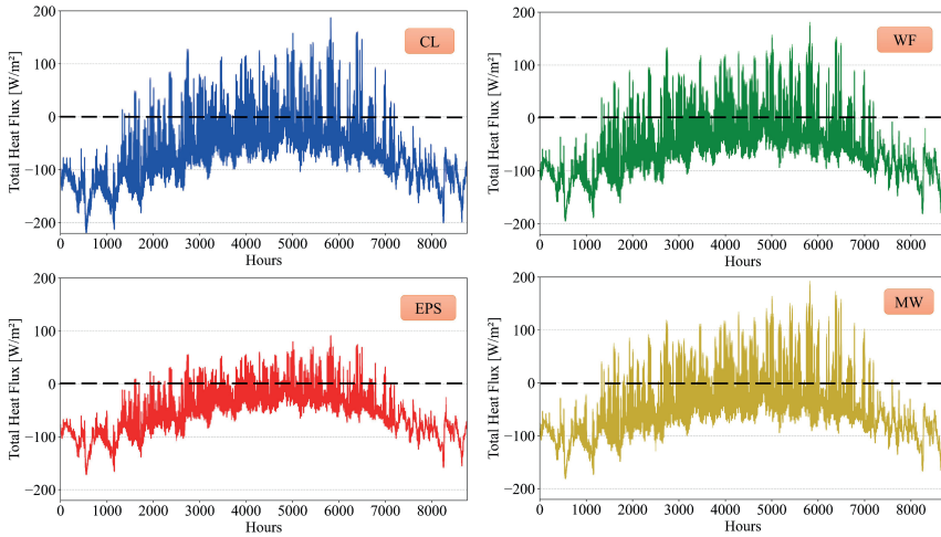
Fig. 5. Total heat flux [ \text{W/m}^2 ]. CL: cellulose, WF: wood fibre, EPS: expanded polystyrene, and MW: mineral wool.
