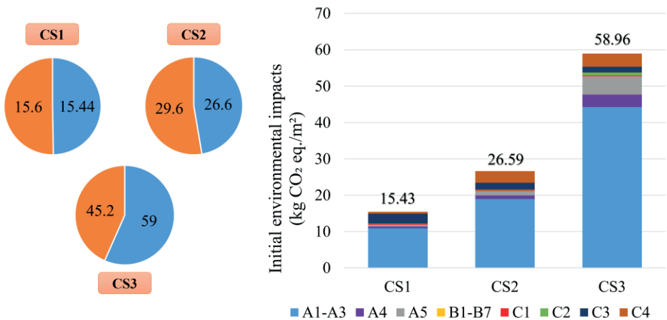
Figure 23: Pie chart: Potential environmental impacts [kg CO 2 eq./m 2 ] of each case study for different building life cycle stages during the lifespan of the building (blue: initial design, orange: over the life span of the building). Bar chart: Initial environmental impacts [kg CO 2 eq./m 2 ] of each case study based on different building life cycle stages and modules.
