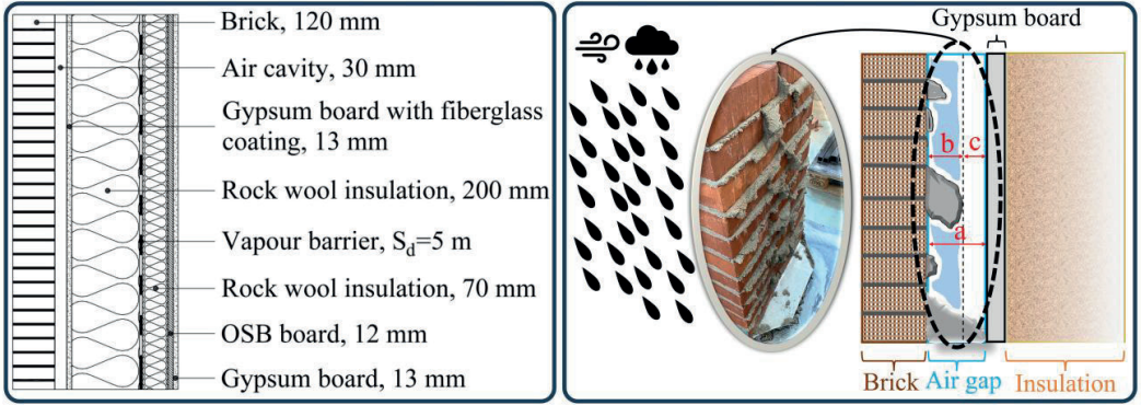
Figure 3: Left : External wall assembly as a case study. Right : Mortar extrusion phenomenon for clay brick cladding (the dimensions are not scaled). a [mm]: whole air gap thickness, b [mm]: extruded mortar thickness, c [mm]: net air gap thickness. Grey clouds: extruded mortar. Blue clouds: existing air between extruded mortar.
