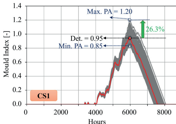
Figure 9: Temporal variation of mould index for a case study (CS1) in Paper II [172], shown for the deterministic case (red line) and the probabilistic analysis (grey region). Abbreviations: Det.: deterministic hygrothermal analysis result, Max. PA and Min. PA: maximum and minimum values of the maximum mould indices according to the probabilistic hygrothermal analysis.
