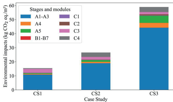
Fig. 7. Initial environmental impacts of each case study based on different building life cycle stages and modules.
