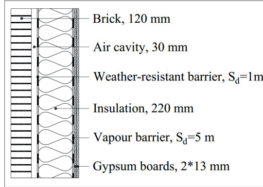
Fig. 2. External wall assembly as the general configuration of the case studies.
