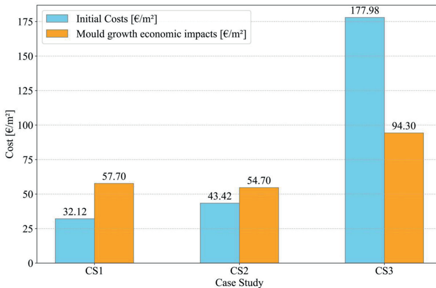
Fig. 6. Potential economic impacts of each case study for different building life cycle stages during the lifespan of the building.
