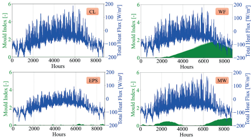
Figure 11: Mould index [-] and total heat flux [ \text{W/m}^2 ]. CL: cellulose, WF: wood fibre, EPS: expanded polystyrene, and MW: mineral wool.
