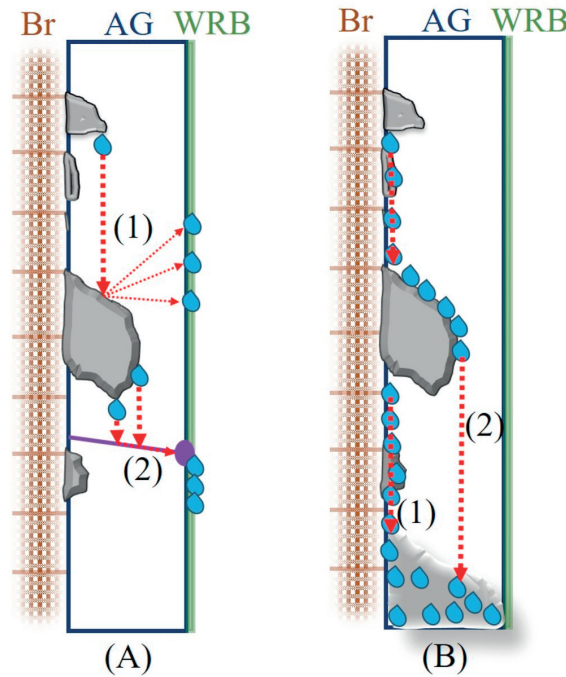
Fig. 12. Possible water penetration scenarios through the extruded mortar. Br: brick layer, AG: airgap layer, and WRB: weather-resistant barrier layer.
