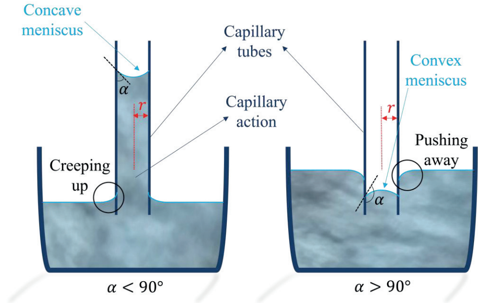
Figure 3: Capillary phenomena in cylindrical capillaries (schematic drawing). Left : Water creeps up the pore wall, giving a contact angle of 0^\circ to 90^\circ . Right : Water is pushed away from the pore wall, giving a contact angle of 90^\circ to 180^\circ .
