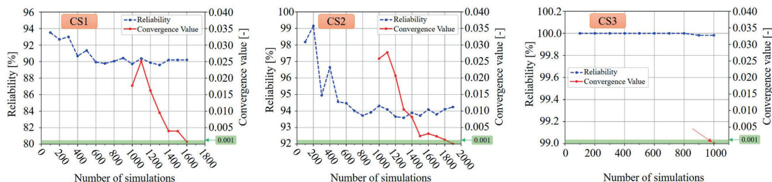
Fig. 5. Required number of scenarios in primary sampling part, as identified by convergence study for three case studies (CS1, CS2, and CS3). Note that convergence of CS3 was obtained already after 10 iterations, as indicated by the red arrow. (For interpretation of the references to colour in this figure legend, the reader is referred to the Web version of this article.)
