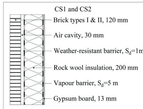
Fig. 3. Two external wall assemblies, case study 1 (CS1) and case study 2 (CS2).
