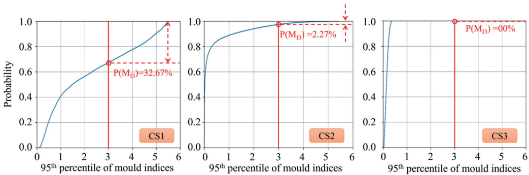
Fig. 5. Mould reliability analysis for three case studies (CS1, CS2, and CS3). Red solid line: failure threshold indicators; blue curve: CDF of 95 th percentile of mould indices; red dashed line: probability of mould index 3 occurrence P(M_{13}) . (For interpretation of the references to colour in this figure legend, the reader is referred to the Web version of this article.)
