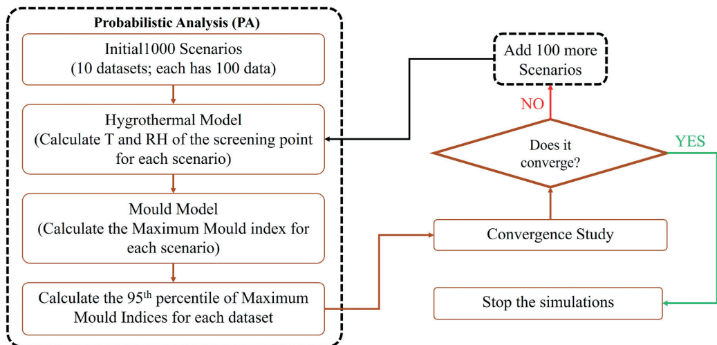
Fig. 1. Probabilistic mould growth analysis procedure.
