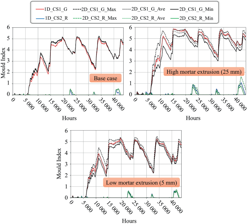
Fig. 6. Wall assemblies modelling for verification, 1D versus 2D. G: Gothenburg, R: Rensjön, CS1: case study 1, CS2: case study 2, Max/Min/Ave: maximum/minimum/average mould index within the 1 m height of the wall in the 2D model.
