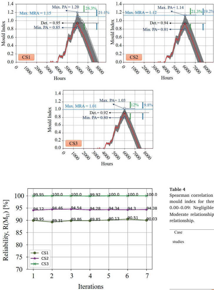
Fig. 8. Reproducibility check with seven iterations for three case studies (CS1, CS2, and CS3).
