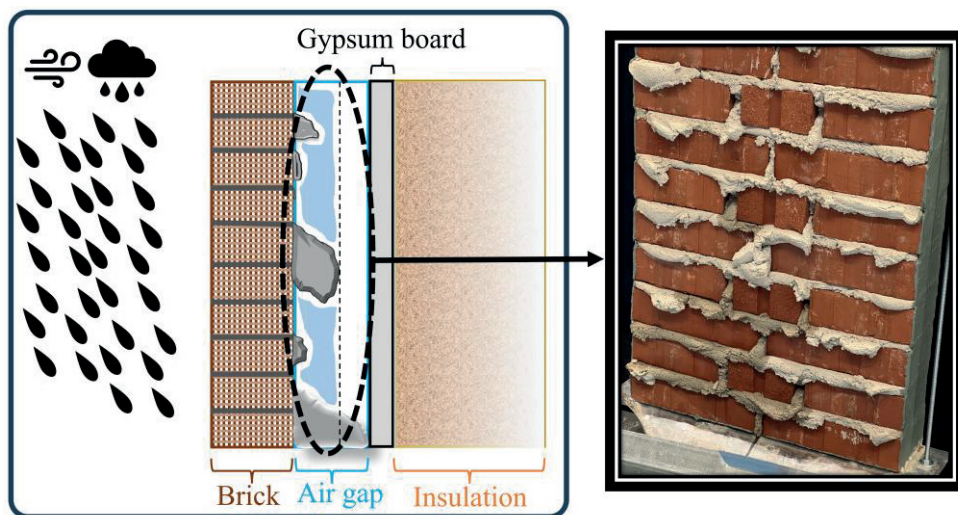
Figure 10: Mortar extrusion phenomenon for clay brick cladding (the dimensions are not scaled).
