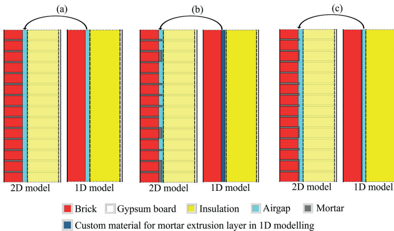
Fig. 5. 1D versus 2D modelling for hygrothermal model verification. (a) Base case, (b) high mortar extrusion (25 mm), and (c) low mortar extrusion (5 mm).
