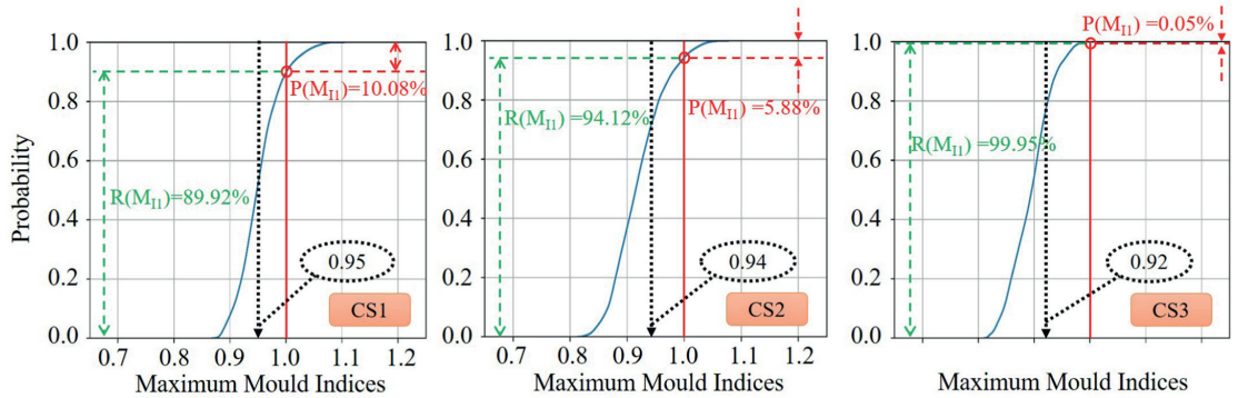
Fig. 6. Mould reliability analysis for three case studies (CS1, CS2, and CS3). Red line: failure threshold indicators; black dotted line: deterministic results; blue line: CDF of maximum mould indices; red dashed line: probability of mould index one occurrence P(M_{I1}) ; green dashed line: reliability of mould index one occurrence R(M_{I1}) . (For interpretation of the references to colour in this figure legend, the reader is referred to the Web version of this article.)
