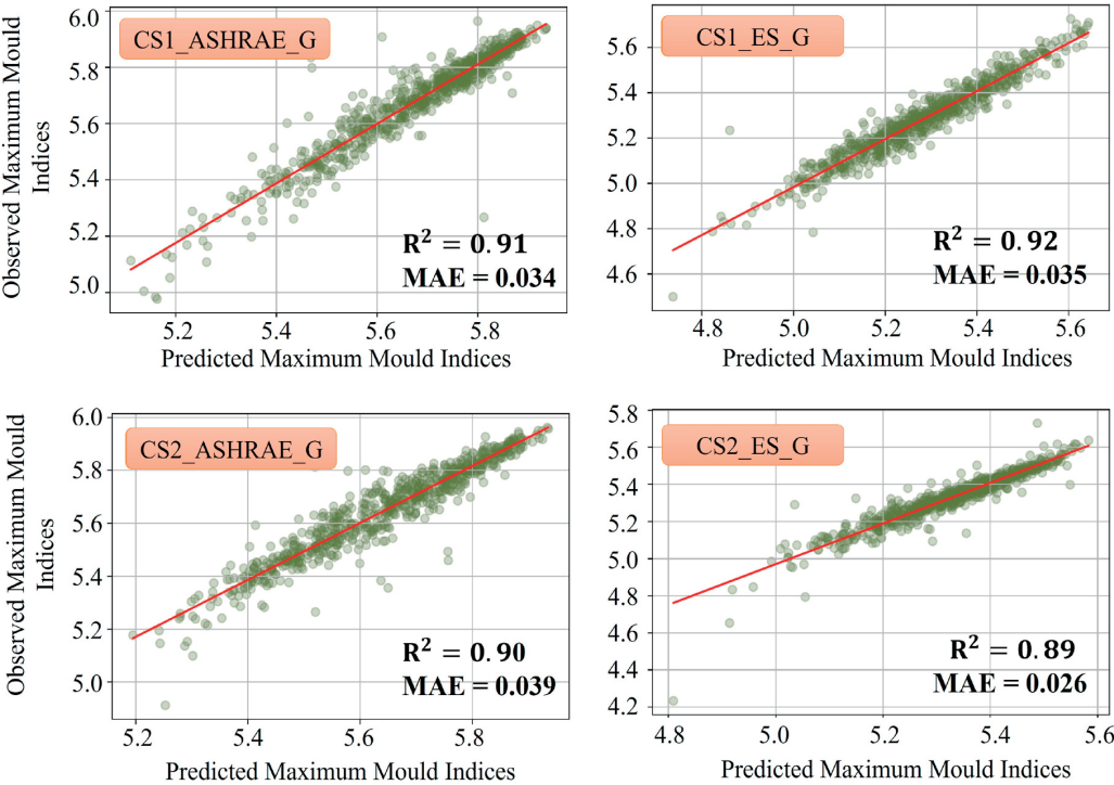
Fig. 7. Predicted vs observed data during the machine learning model testing, Gothenburg (G). ES: case studies (CS1 and CS2) based on experimental study data.
