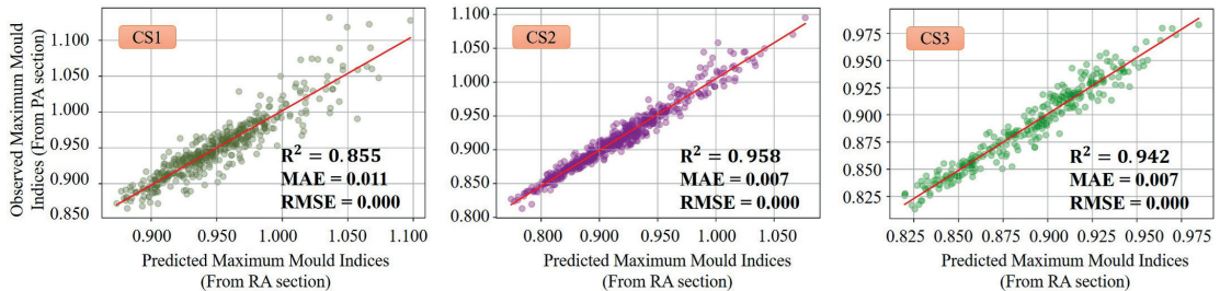
Fig. 4. Predicted data (from RA section) vs observed data (from PA section) during the machine learning model testing for three case studies (CS1, CS2, and CS3).
