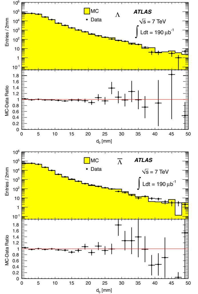
FIG. 5 (color online). The distribution of the reconstructed transverse impact parameter in 7 TeV data and MC for protons and antiprotons originating in \Lambda (top) and \bar{\Lambda} decays (bottom) with p_T > 500 MeV after all selection criteria are imposed.
