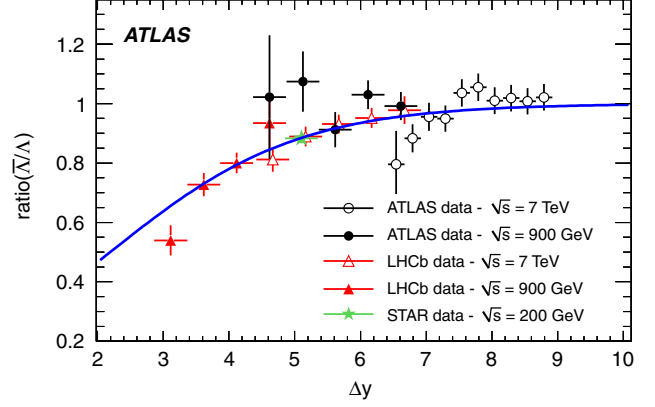
FIG. 24 (color online). The production ratio between \bar{\Lambda} and \Lambda baryons measured by ATLAS and other experiments versus the rapidity difference with respect to the beam. The error bars on the ATLAS data show statistical and systematic uncertainties added in quadrature. The solid line shows the fit to all data points described in the text.
