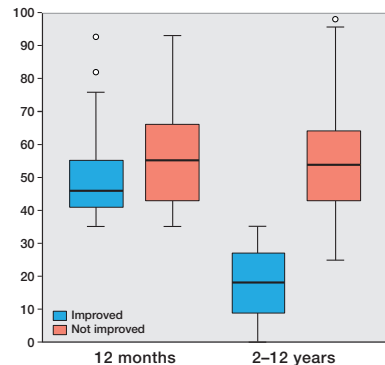
DASH score
