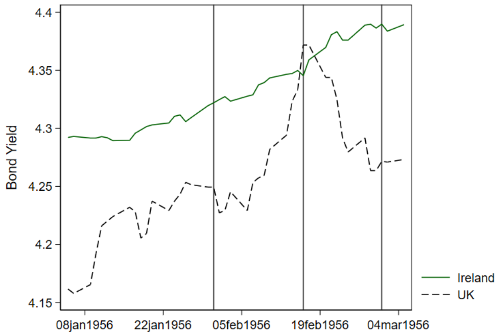
Figure 18: Anticipation effects
