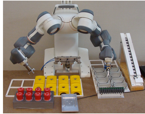
(a) The parts that are used in the process: the bottom of an emergency stop box (later "box") and a switch that will be inserted into the box. (b) The two-armed ABB robot and the workspace setup.
