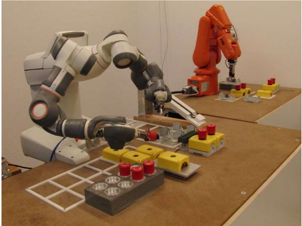
Figure 8: A setup of two different robots, the two-armed concept robot Frida and the ABB IRBr20, for individual or coordinated assembly of emergency buttons within the ROSETTA project.
