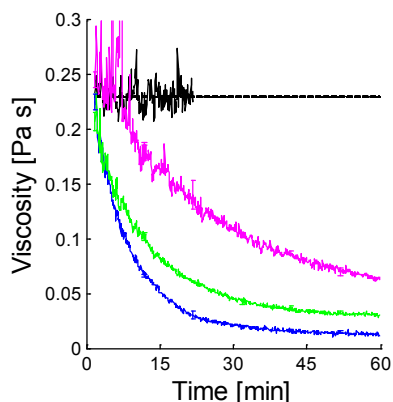
Figure 3.8. In situ viscosity at a shear rate of 160.7 \text{ s}^{-1} during enzymatic hydrolysis of sulfite pretreated spruce (2% WIS), as reported in Paper II . Black denotes biomass without enzyme addition, while blue and green denote hydrolysis at a protein loading of 10.4 \text{ mg}_{\text{prot}}/\text{g}_{\text{gluc}} , of Cellic CTec3 or an endoglucanase preparation, respectively. Magenta denotes endoglucanase hydrolysis at 1.04 \text{ mg}_{\text{prot}}/\text{g}_{\text{gluc}} .
