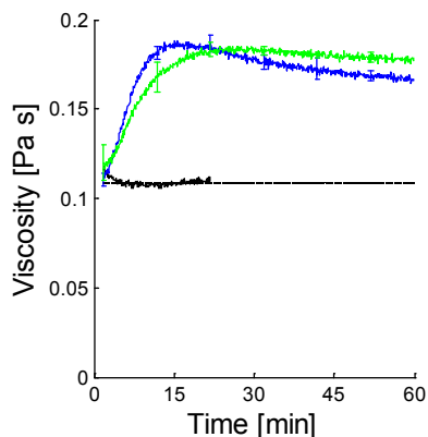
Figure 3.7. In situ viscosity at a shear rate of 160.7 \text{ s}^{-1} during enzymatic hydrolysis of batch steam pretreated pine (12% WIS), as reported in Paper II . Black denotes biomass without enzyme addition, while blue and green denotes hydrolysis at a protein loading of 10.4 \text{ mg}_{\text{prot}}/\text{g}_{\text{gluc}} , with Cellic CTec3 or an endoglucanase preparation, respectively.
