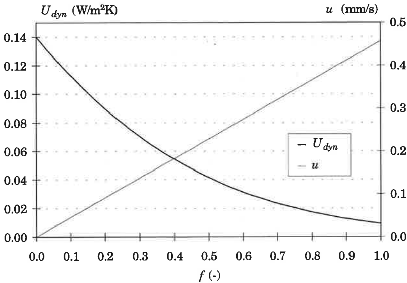
Figure 3.1 The dynamic U value according to (3.7) and the flow u as a function of the proportion, f , of the inlet air that passes through the dynamic insulation ( H=0.3m ).
