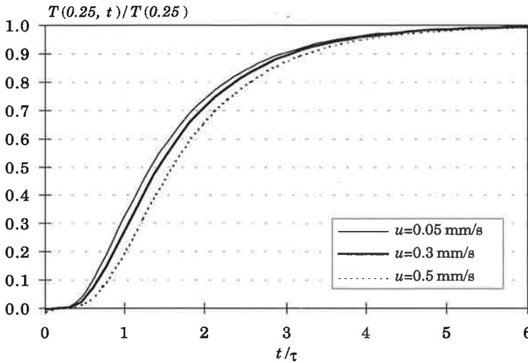
Figure 2.1 The ratio of the transient to the steady state temperature for u=0.05 - 0.5 mm/s, ( x=0.25 m) as a function of t/\tau .
