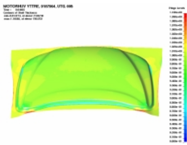
Figure 5. Thickness distribution.
