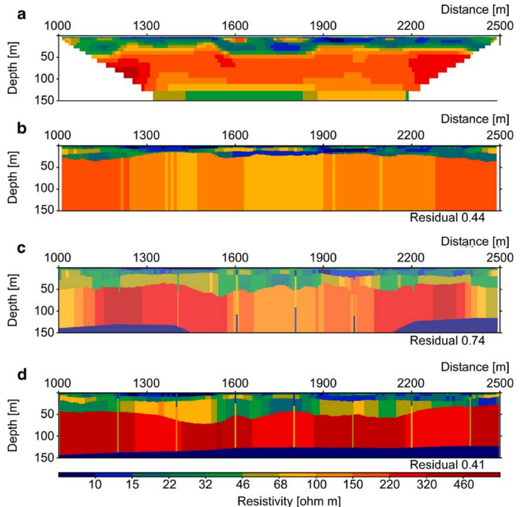
Fig. 6 Test profile used to determine the set-up of constraints. In a it is the two-dimensional inversion of CVES data by Res2dinv is shown, in b it is the one-dimensional LCI of CVES data, in c it is an abandoned attempt of LCI of TEM and CVES data, whereas d is the LCI with the model as chosen. A residual of 1 corresponds to a fit at the uncertainty applied to the data. Hence, data are fitted within the data uncertainty
