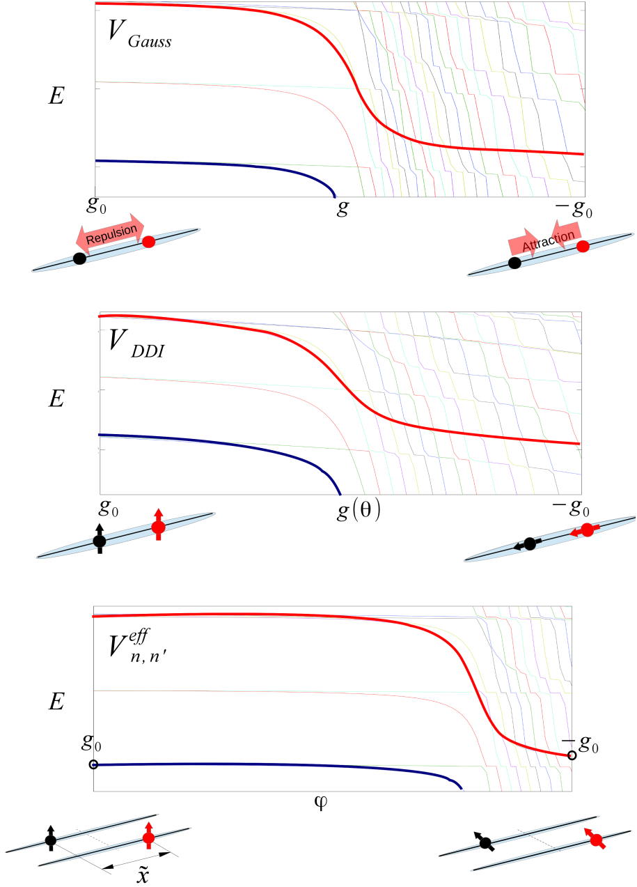
Figure 30: A schematic view of the different energy spectra for two particles in a quasi 1D harmonic trap. The spectra are sketched for three different interaction pseudopotentials; V_{Gauss} in Eq. (18), V_{DDI} in Eq. (19), and V_{n,n'}^{eff} in Eq. (16). Here, g represents the peak value of each potential V(0) = g . The spectra all have a similar structure.
