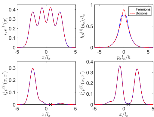
FIG. 5: (Color online) Similar to Fig. 4 but for \phi = 0.91 \approx 52.14^\circ , which corresponds to a repulsive inter-trap interaction.
