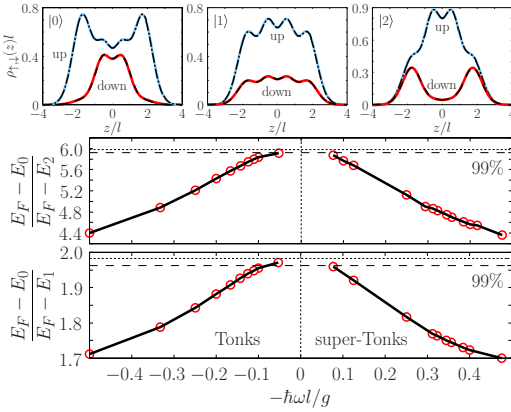
FIG. 7. (Color online) The same as Fig. 6 for the ( N_t = 3, N_l = 1 ) system. Top: Spin densities of the effective spin-chain model (solid lines) and of an exact diagonalization of the full Hamiltonian for g/(ħωl) = 25 in a harmonic trap (dashed and dash-dotted lines). Bottom: Ratio of energy differences of the ground-state multiplet as a function of -1/g [solid (black) line with (red) circles]. The corresponding values of the spin-chain model are 1.982 and 5.983, respectively (horizontal short-dashed lines). The horizontal long-dashed lines mark -1\% deviation from these values.
