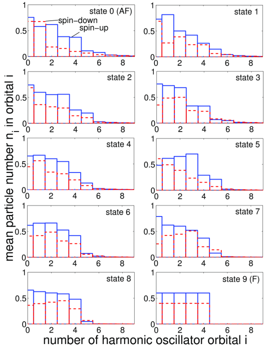
FIG. 8. (Color online) Mean occupation numbers \langle n_i \rangle of the harmonic-oscillator orbitals of an ( N_t = 3, N_l = 2 ) Fermi system in the Tonks regime [ g/(ħωl) = 30 , ground-state multiplet].
