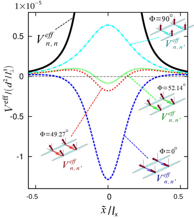
Figure 21: Effective DDI, approximated by Eq. (16) for different angular configurations of the double trap system, as a function of the relative coordinate \tilde{x}/l_x . The short-range part of V_{n,n'}^{\text{eff}} can be changed toward positive or negative values by tuning \phi , as sketched in the insets. This figure is taken from paper v.
