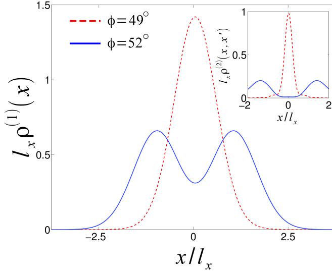
Figure 22: Single-particle density \rho_{T_n} + \rho_{T_{n'}} for the ground state of a doubletrap system with one particle in each trap. The densities are plotted for two different dipolar angles, \phi = 49^\circ and \phi = 52^\circ . Inset: Pair-correlated densities for a reference particle at x = 0 . For \phi = 49^\circ the attractive part of V_{n,n'}^{\text{eff}} produces a bound dimer with high probability of finding two particles at the same position. For \phi = 52^\circ the repulsive parts of V_{n,n'}^{\text{eff}} produces a separated state with very small probability of finding two particles at the same position.
