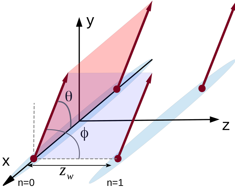
Figure 20: Sketch of two quasi 1D harmonic traps with four dipolar particles. The direction of the dipole moments are indicated by the red arrows, with directions defined by the two angles \theta and \phi . The distance between the traps is denoted by z_w . This figure is taken from paper V.
