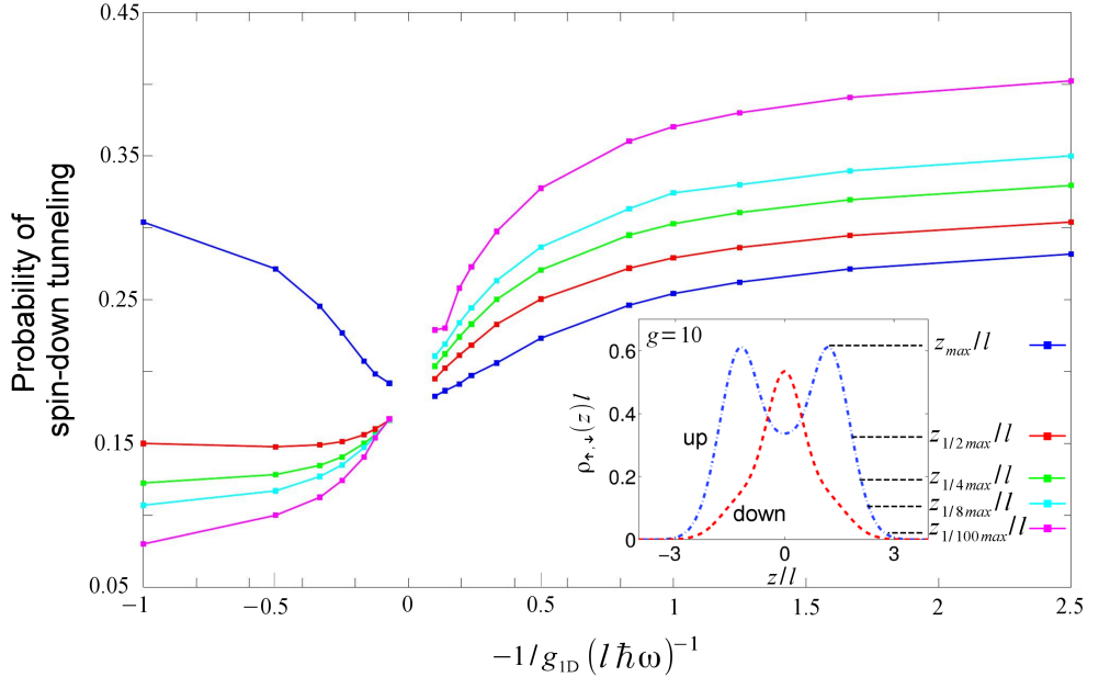
Figure 8: Numerically calculated spin-down fractions, \rho_{\downarrow}(z)/(\rho_{\uparrow}(z)+\rho_{\downarrow}(z)) (i.e., the fraction between the single-particle spin-down density and the total single-particle density), for the 2+1 AF state at different interaction strengths g_{1D} . Inset: Single-particle densities of spin-up and spin-down particles with indications of the positions in z at which the spin-down fraction is calculated. The overall curve matches well with experiments only for positions far right of the trap center.
