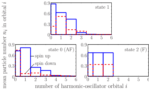
FIG. 5. (Color online) Mean occupation \langle n_i \rangle of the harmonic-trap levels for the (N_\uparrow = 2, N_\downarrow = 1) system in the Tonks regime [g/(h\omega) = 25] for the states |0\rangle , |1\rangle , and |2\rangle (see text) of the ground-state multiplet.
