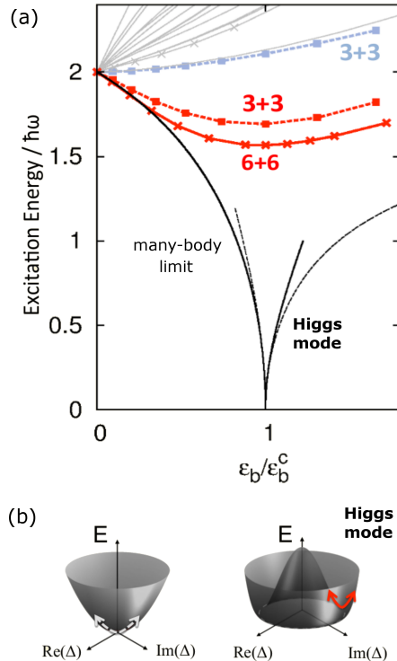
Figure 14: Numerical excitation energies for 3+3 fermions (dashed red line) and for 6+6 fermions (red solid line) obtained in the L = 0 subspace (the energy for 6 + 6 fermions is an upper bound). The blue dashed line is the second excited state. The solid gray lines are higher excitations for the 3 + 3 system. The black solid (dotted) lines show the results of the numerical (analytic) many-body calculations of a sharp Higgs mode in [111]. This figure is taken from paper I.
