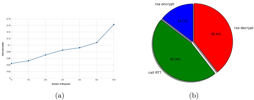
Figure C.1: Performance evaluation: (a) Time required by TTP to process a request and to generate a key for a domain; (b) Proportion of execution time spent in functions during a key request.
