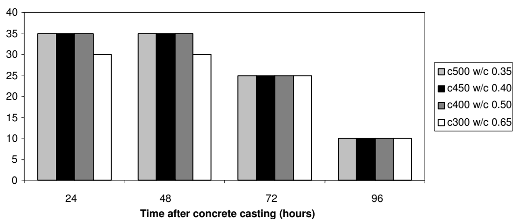
Figure 6.13 Used concrete temperature data during the first four days, based on calculations through the PC-program Hett97 (1997) for the surrounding air temperature of Climate 5. Used cement content between 300 kg/m 3 (c300) and 500 kg/m 3 (c500). Cast slab thickness 0.20 m, Filigran-form, concrete temperature at casting 20°C, infra heating (350 W/m 2 ) during the first 24 hours and 'high-quality' covering (definition according to Hett97).
