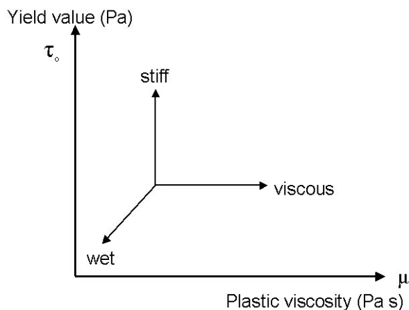
Figure 3.8 In contradiction to viscosity, properties as ‘stiffness’ and ‘wetness’ are affected by the yield value according to Wallevik (2003).
