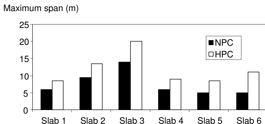
Figure A.8. Comparison between normal house-building concrete (NPC) and high performance concrete (HPC) with regard to maximum slab span allowed in all studied slab types.
