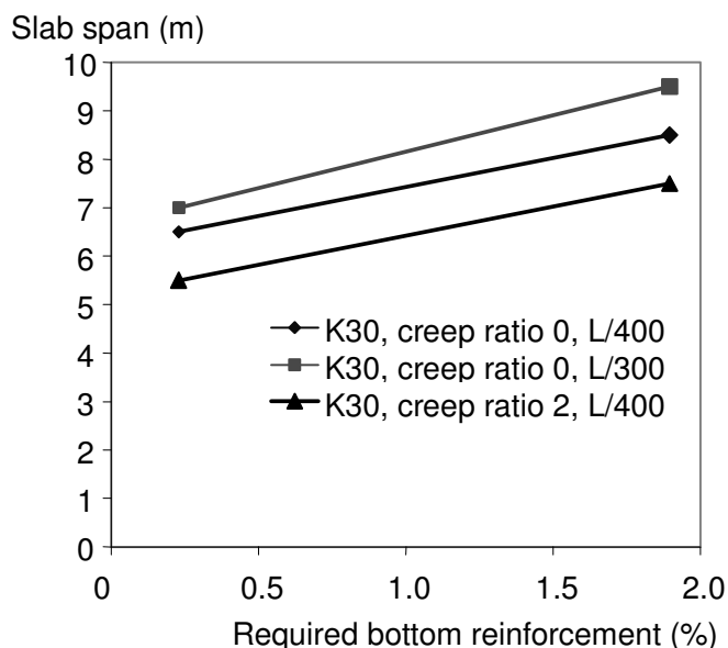
Figure A.17 Estimated influence of increased concrete creep ratio (from 0 to 2) and decrease of the deformation criteria (from L/400 to L/300 ) on the maximum slab span allowed for slab type 1. Concrete quality K30.
