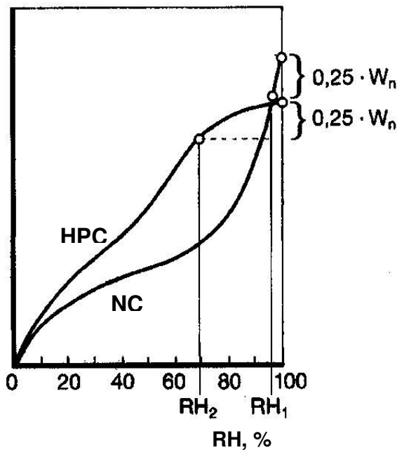
Figure 6.5 Sorption isotherm of HPC compared to NC-principles (Fagerlund, 1994). 0.25 W_n is the amount of self-desiccated pores where W_n is the amount of chemically bound water (kg/m 3 ).
