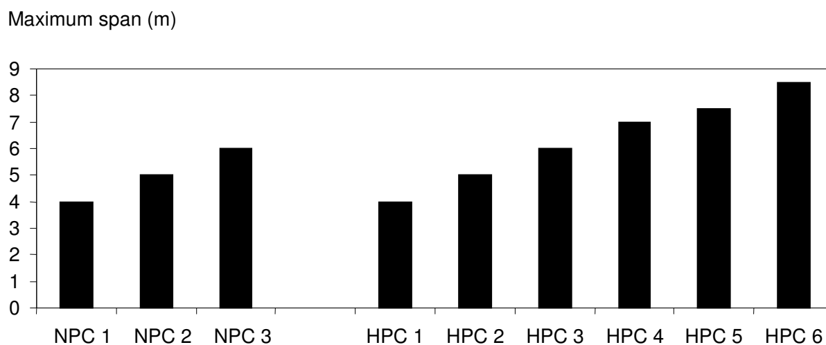
Figure A.9 Effects of various concrete and slab parameters on maximum slab span. Slab type 1.
