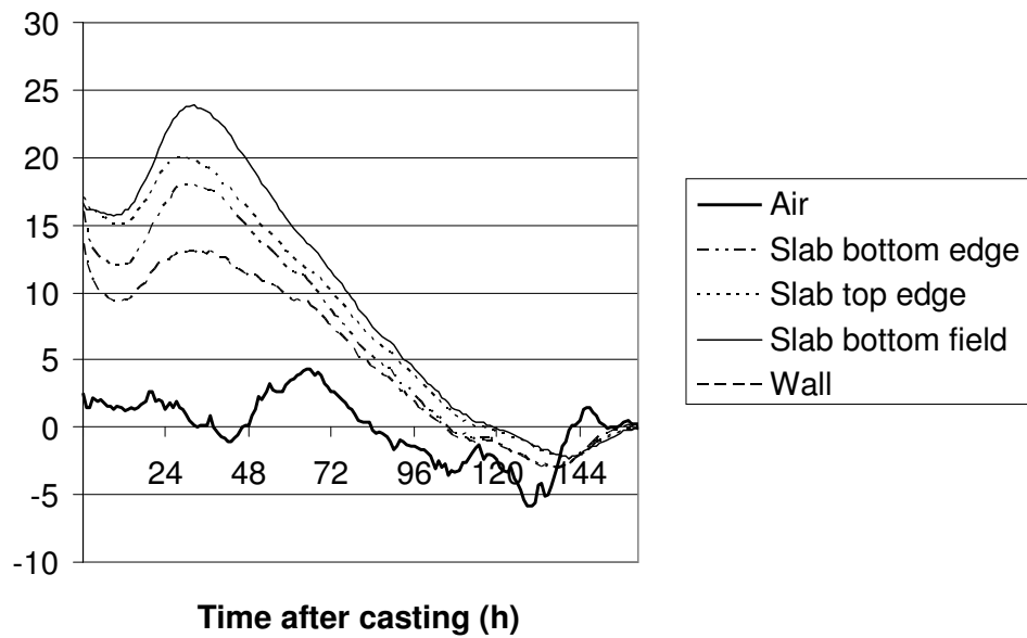
Figure 4.2a Example of measured temperature development in SCC on site in Case 3 using maturity meters.
