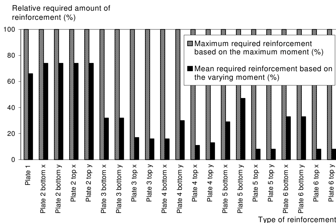
Figure A.16 Comparison between required reinforcement based on the maximum and the average slab moment.
