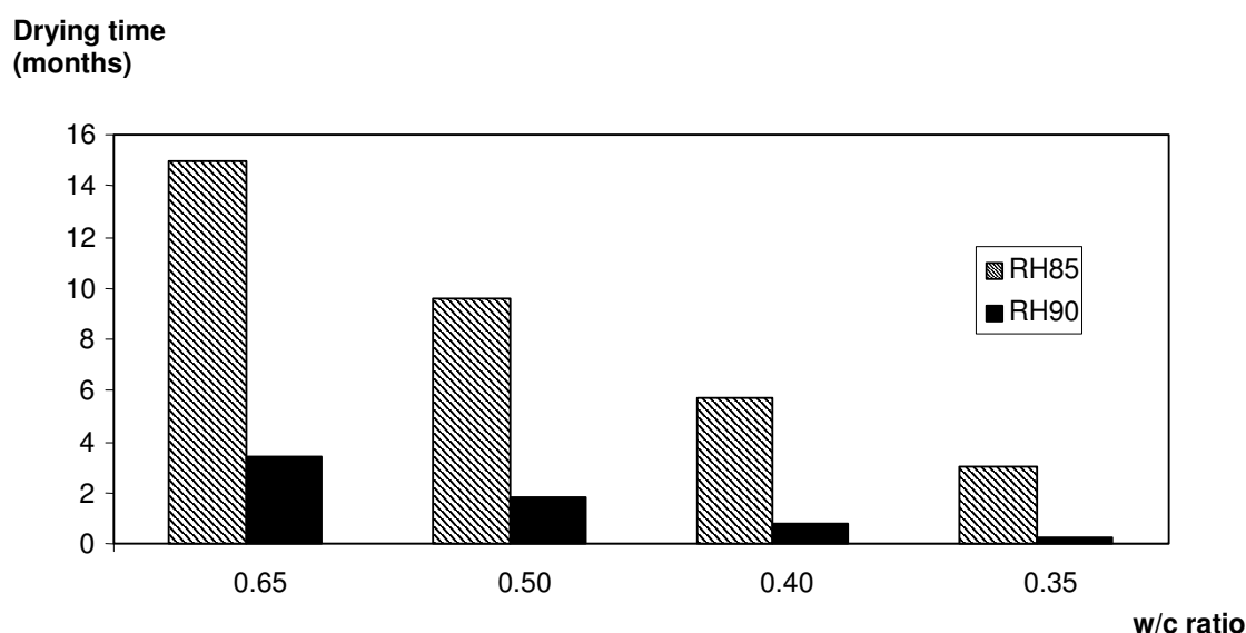
Figure 6.8 Required drying time for reaching 85 and 90% RH at the equivalent depth (for definition, see above) as function of w/c ratio. Data are taken from section 6.2. The result is based on calculations based on the PC-program TorkaS 1.0 (1998). Conditions are slab thickness 0.20 m, double-sided drying and controlled drying climate (air RH 60% and air temperature 18 °C) from the start of casting.
