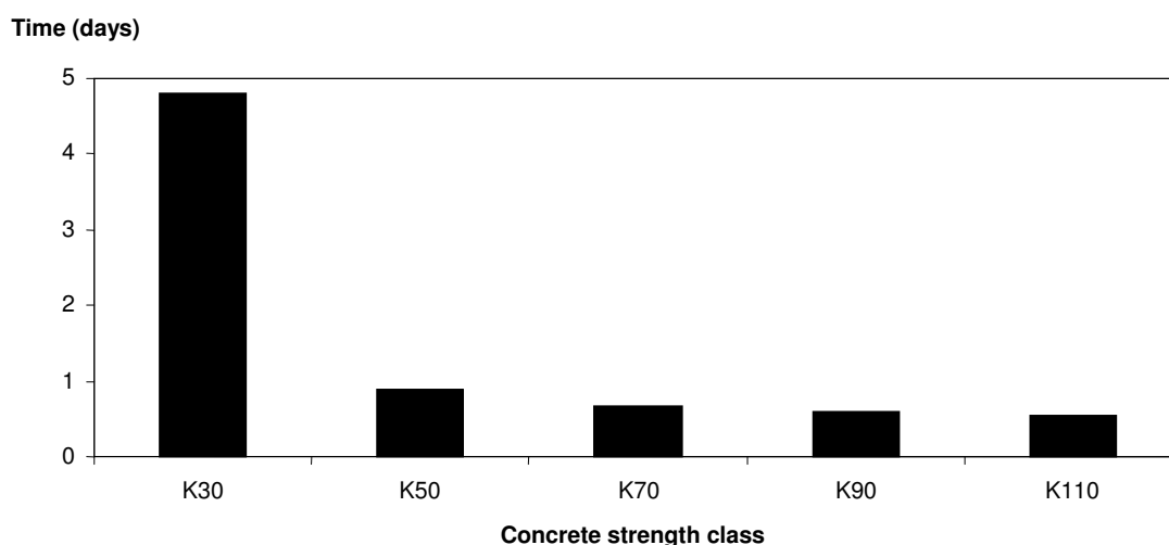
Figure 6.18 Calculated time required for reaching 20 MPa minimum strength at the slab top surface for various concrete strength classes during summer conditions, (+15 °C). 19 mm plywood form.
