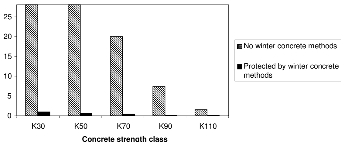
Figure 6.21 Calculated time to reach 20 MPa at outer temperature of -5°C. Effect of winter precaution activities is regarded. 19 mm plywood form. Concrete temperature at casting +20°C.
