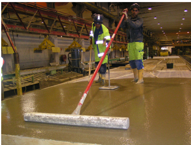
Figure 5.7 SCC full-scale casting simulating 'real' conditions.
