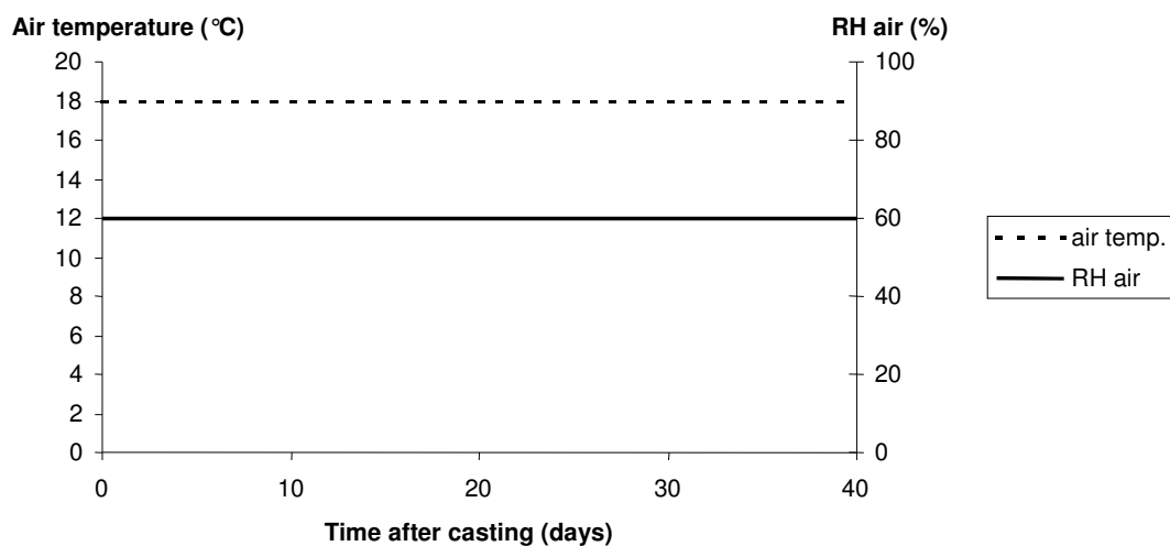
Figure 6.2 Surrounding climate conditions for Climate 1 during the first 40 days after concrete casting.
