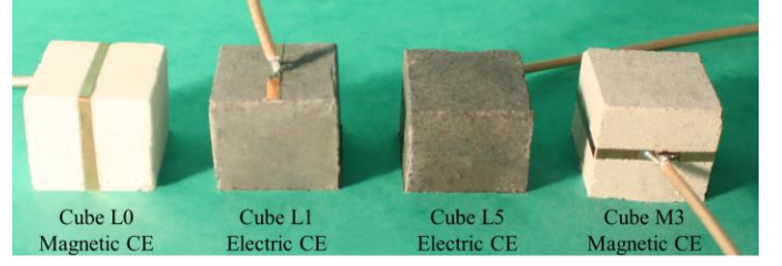
Fig. 11. Four of the eight physical prototypes that were fabricated. Two of the structures show how the electric CE was implemented, while the other two structures show how the magnetic CE was implemented.
